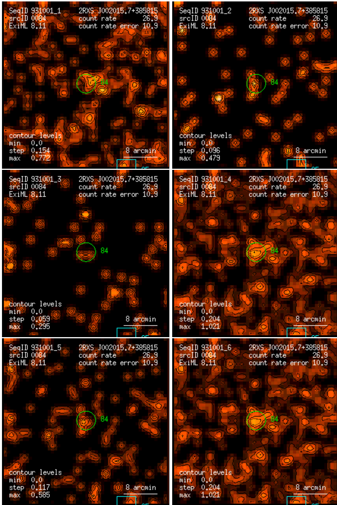
Figure 84: RASS 931001: detection 0084: band rate images, Gaussian filter: (1) PSPC channels 11 – 41, (2) 52 – 90, (3) 91 – 201, (4) 11 – 235, (5) 52 – 201, (6) 11 – 201. Broad band rates in counts/ks. Band rate contour levels in counts/ks/arcmin 2 .
