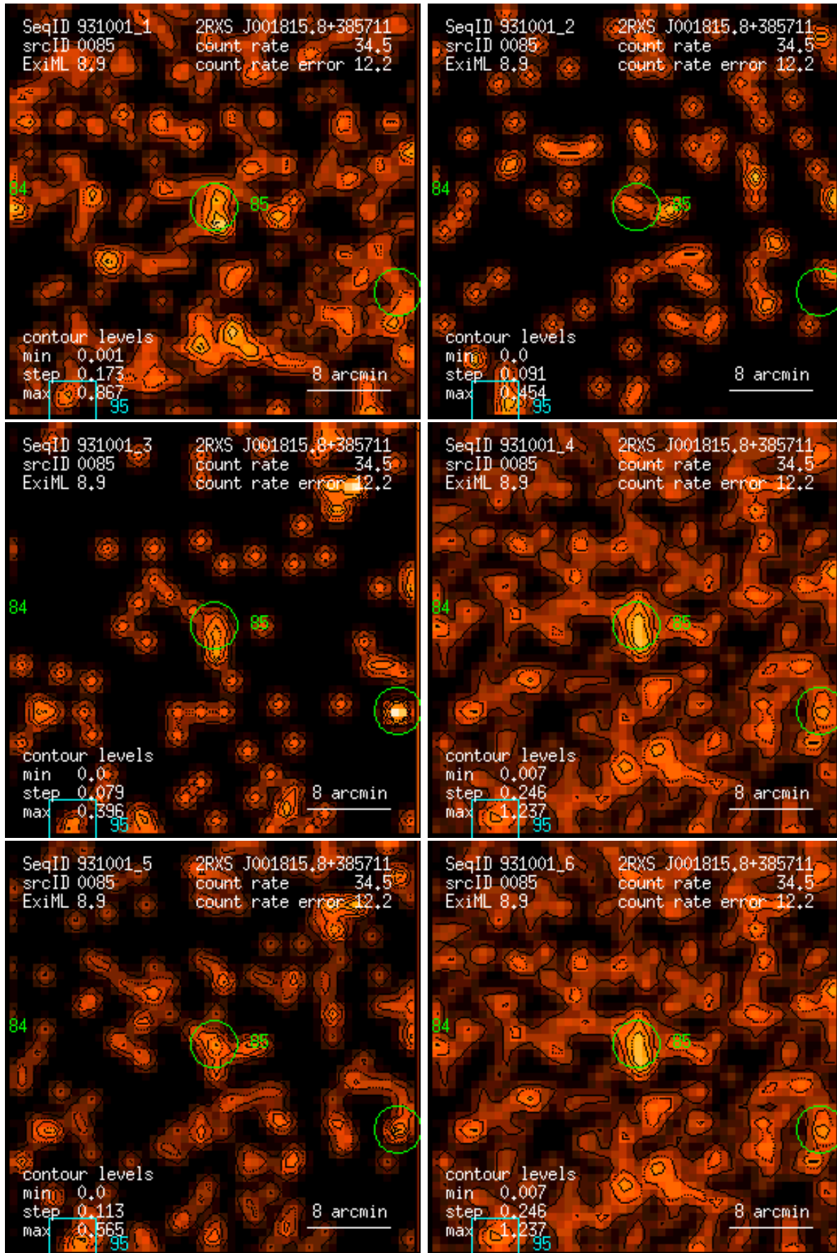
Figure 85: RASS 931001: detection 0085: band rate images, Gaussian filter: (1) PSPC channels 11 – 41, (2) 52 – 90, (3) 91 – 201, (4) 11 – 235, (5) 52 – 201, (6) 11 – 201. Broad band rates in counts/ks. Band rate contour levels in counts/ks/arcmin 2 .
