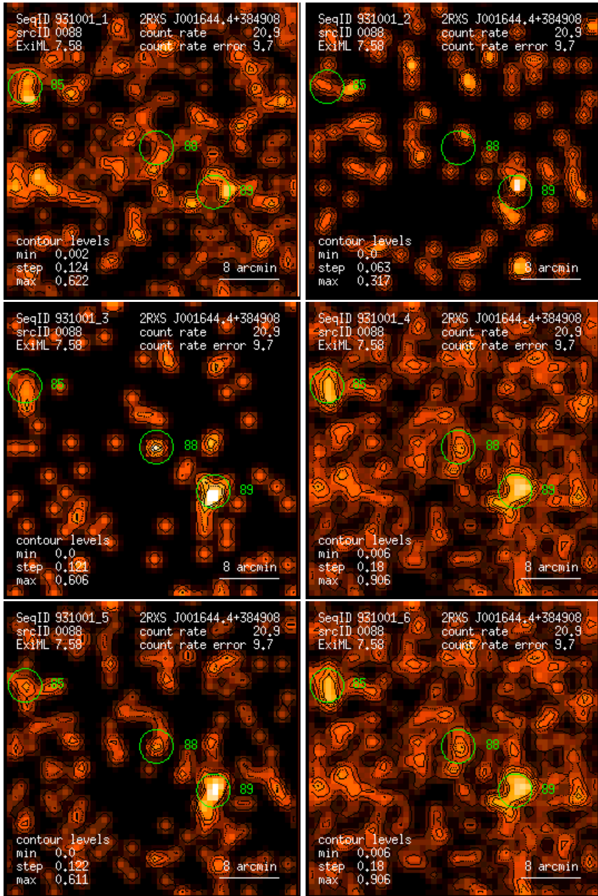
Figure 88: RASS 931001: detection 0088: band rate images, Gaussian filter: (1) PSPC channels 11 – 41, (2) 52 – 90, (3) 91 – 201, (4) 11 – 235, (5) 52 – 201, (6) 11 – 201. Broad band rates in counts/ks. Band rate contour levels in counts/ks/arcmin 2 .
