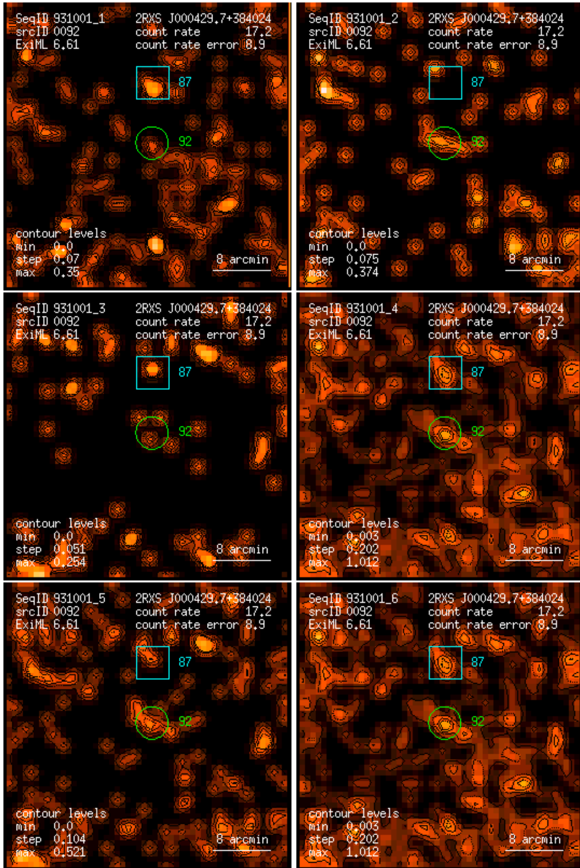
Figure 92: RASS 931001: detection 0092: band rate images, Gaussian filter: (1) PSPC channels 11 – 41, (2) 52 – 90, (3) 91 – 201, (4) 11 – 235, (5) 52 – 201, (6) 11 – 201. Broad band rates in counts/ks. Band rate contour levels in counts/ks/arcmin 2 .
