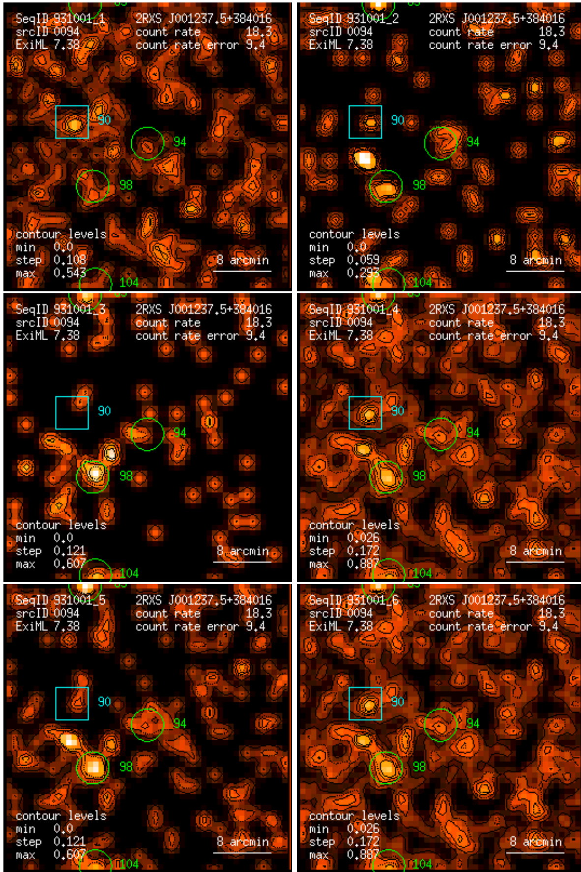
Figure 94: RASS 931001: detection 0094: band rate images, Gaussian filter: (1) PSPC channels 11 – 41, (2) 52 – 90, (3) 91 – 201, (4) 11 – 235, (5) 52 – 201, (6) 11 – 201. Broad band rates in counts/ks. Band rate contour levels in counts/ks/arcmin 2 .
