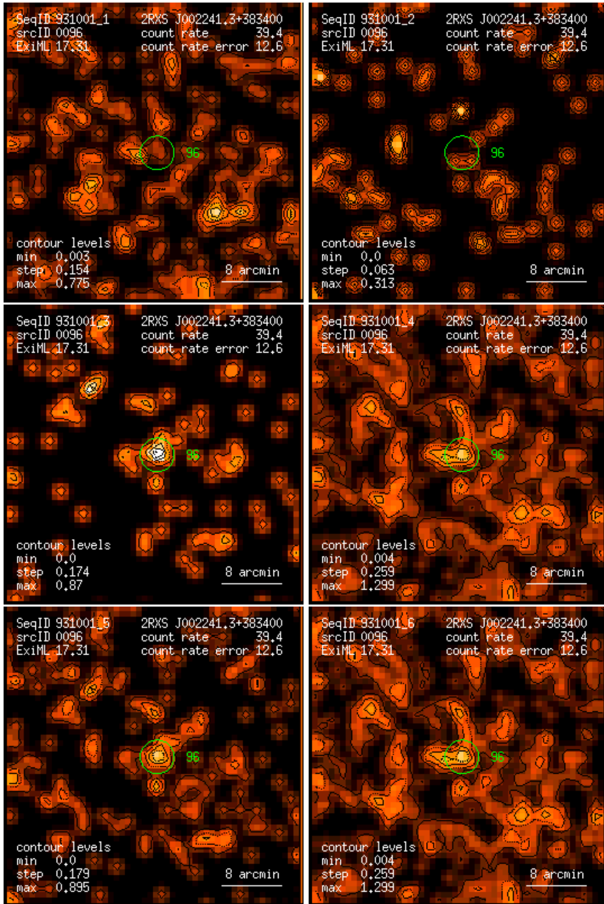
Figure 96: RASS 931001: detection 0096: band rate images, Gaussian filter: (1) PSPC channels 11 – 41, (2) 52 – 90, (3) 91 – 201, (4) 11 – 235, (5) 52 – 201, (6) 11 – 201. Broad band rates in counts/ks. Band rate contour levels in counts/ks/arcmin 2 .
