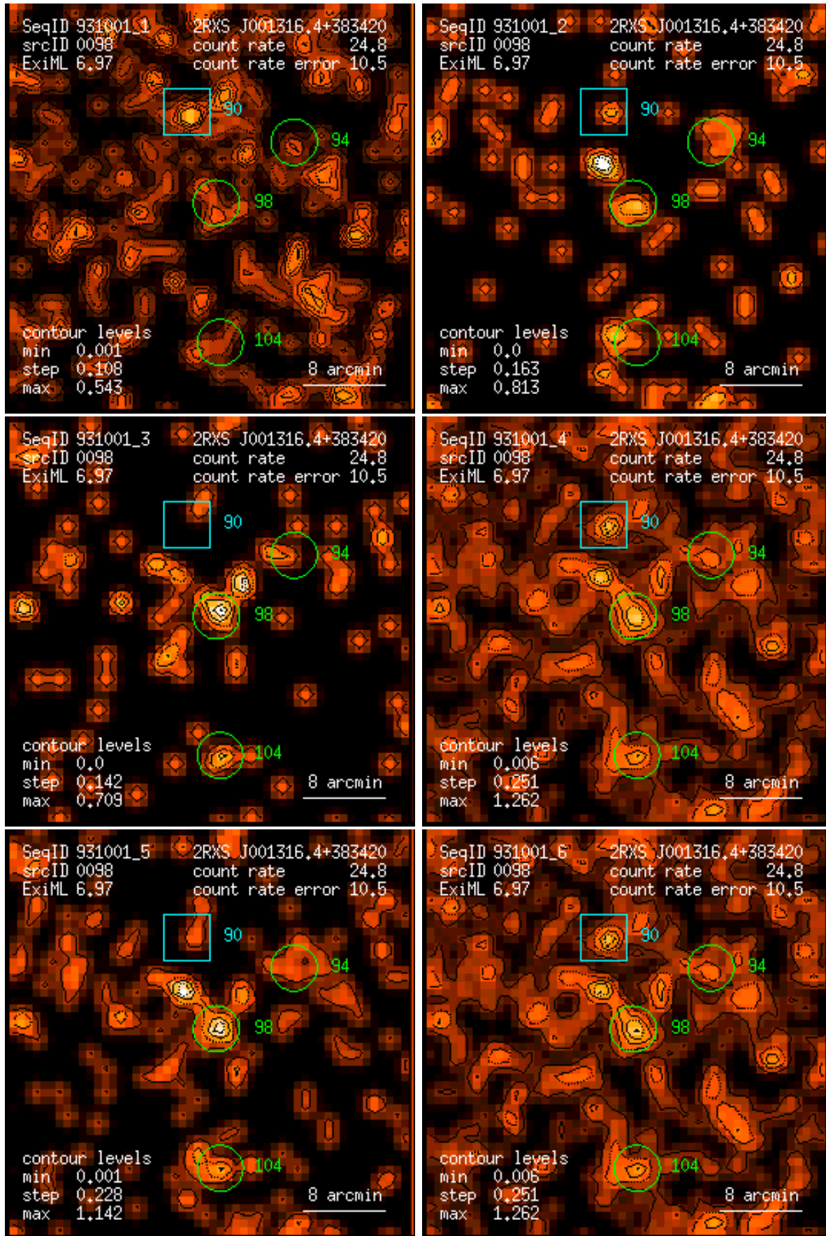
Figure 98: RASS 931001: detection 0098: band rate images, Gaussian filter: (1) PSPC channels 11 – 41, (2) 52 – 90, (3) 91 – 201, (4) 11 – 235, (5) 52 – 201, (6) 11 – 201. Broad band rates in counts/ks. Band rate contour levels in counts/ks/arcmin 2 .
