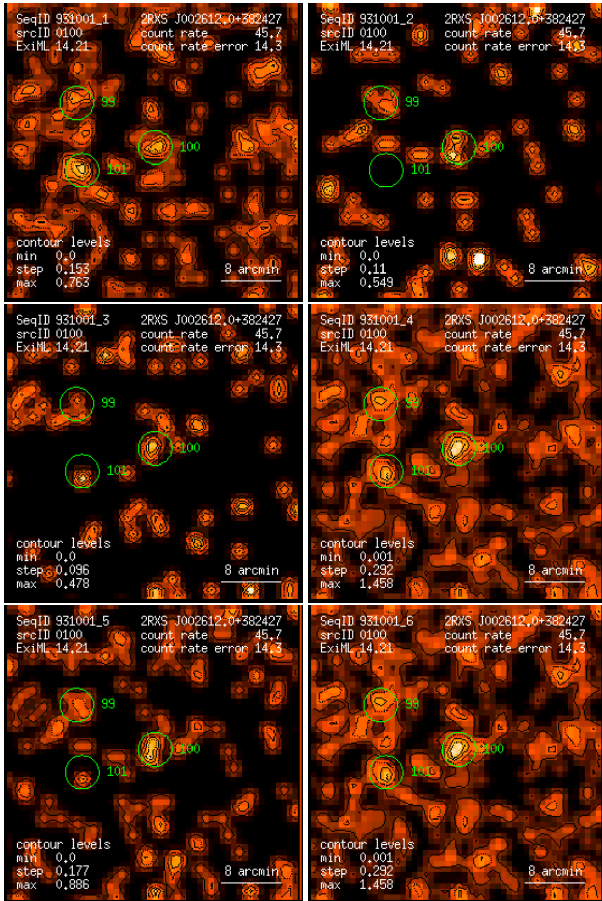
Figure 100: RASS 931001: detection 0100: band rate images, Gaussian filter: (1) PSPC channels 11 – 41, (2) 52 – 90, (3) 91 – 201, (4) 11 – 235, (5) 52 – 201, (6) 11 – 201. Broad band rates in counts/ks. Band rate contour levels in counts/ks/arcmin 2 .
