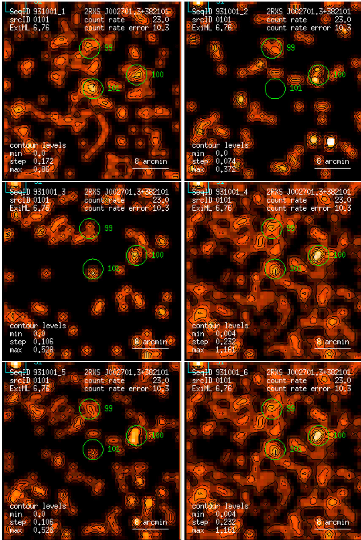
Figure 101: RASS 931001: detection 0101: band rate images, Gaussian filter: (1) PSPC channels 11 – 41, (2) 52 – 90, (3) 91 – 201, (4) 11 – 235, (5) 52 – 201, (6) 11 – 201. Broad band rates in counts/ks. Band rate contour levels in counts/ks/arcmin 2 .
