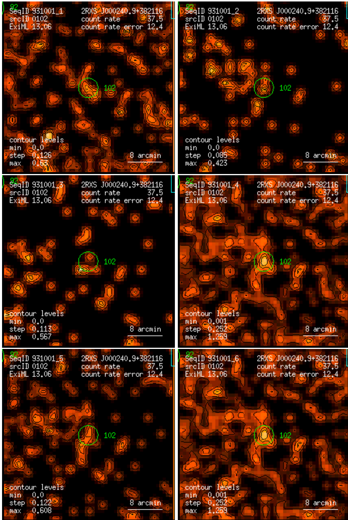
Figure 102: RASS 931001: detection 0102: band rate images, Gaussian filter: (1) PSPC channels 11 – 41, (2) 52 – 90, (3) 91 – 201, (4) 11 – 235, (5) 52 – 201, (6) 11 – 201. Broad band rates in counts/ks. Band rate contour levels in counts/ks/arcmin 2 .
