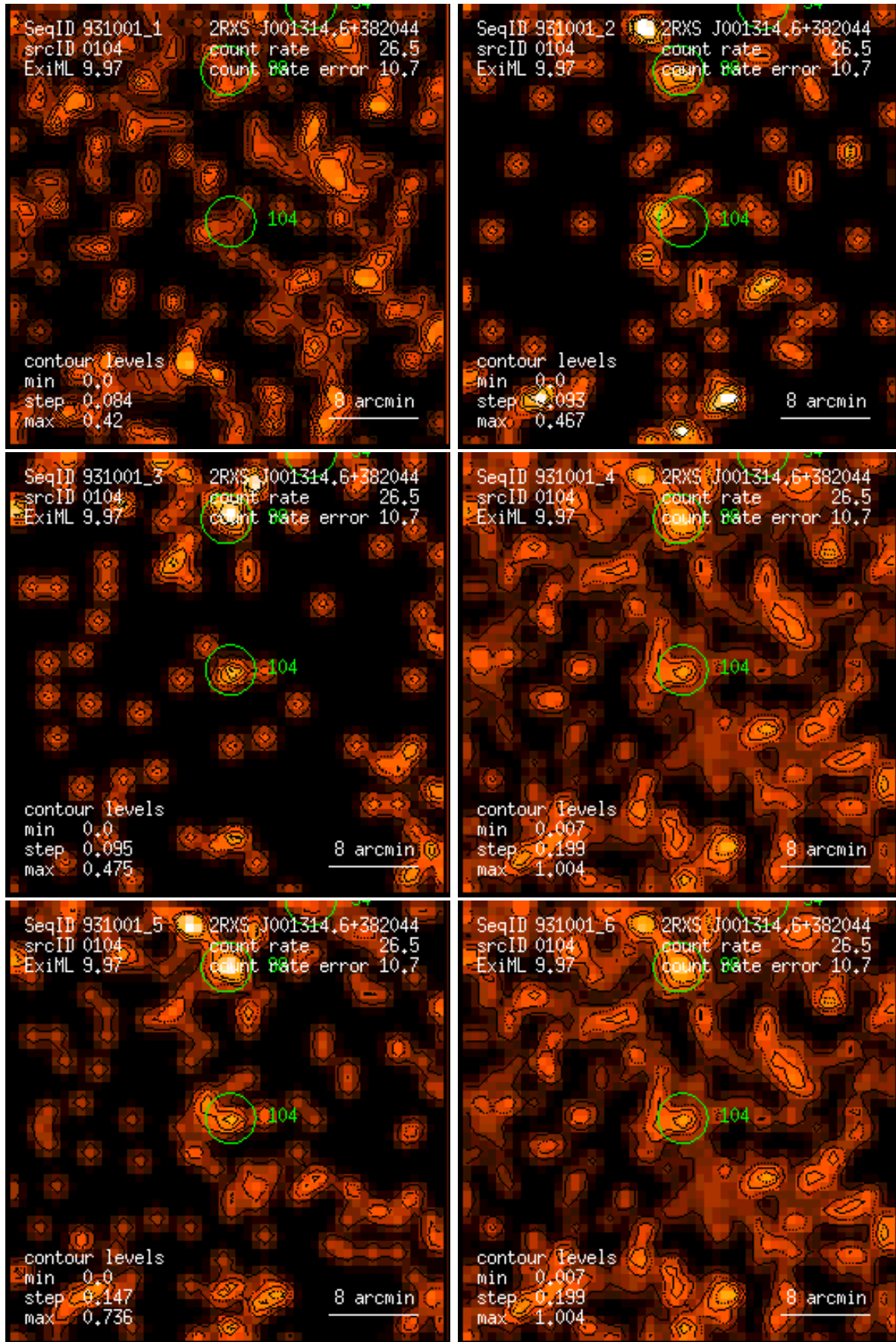
Figure 104: RASS 931001: detection 0104: band rate images, Gaussian filter: (1) PSPC channels 11 – 41, (2) 52 – 90, (3) 91 – 201, (4) 11 – 235, (5) 52 – 201, (6) 11 – 201. Broad band rates in counts/ks. Band rate contour levels in counts/ks/arcmin 2 .
