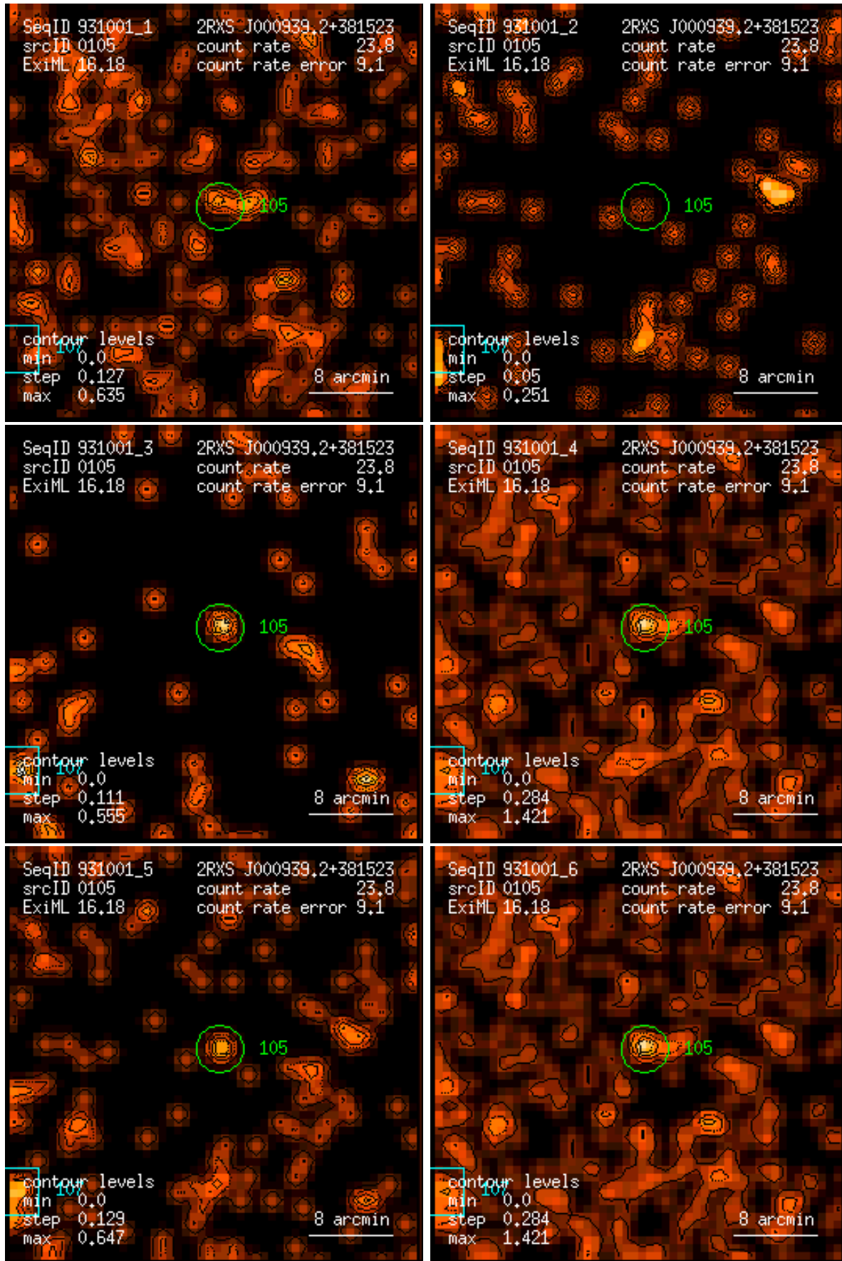
Figure 105: RASS 931001: detection 0105: band rate images, Gaussian filter: (1) PSPC channels 11 – 41, (2) 52 – 90, (3) 91 – 201, (4) 11 – 235, (5) 52 – 201, (6) 11 – 201. Broad band rates in counts/ks. Band rate contour levels in counts/ks/arcmin 2 .
