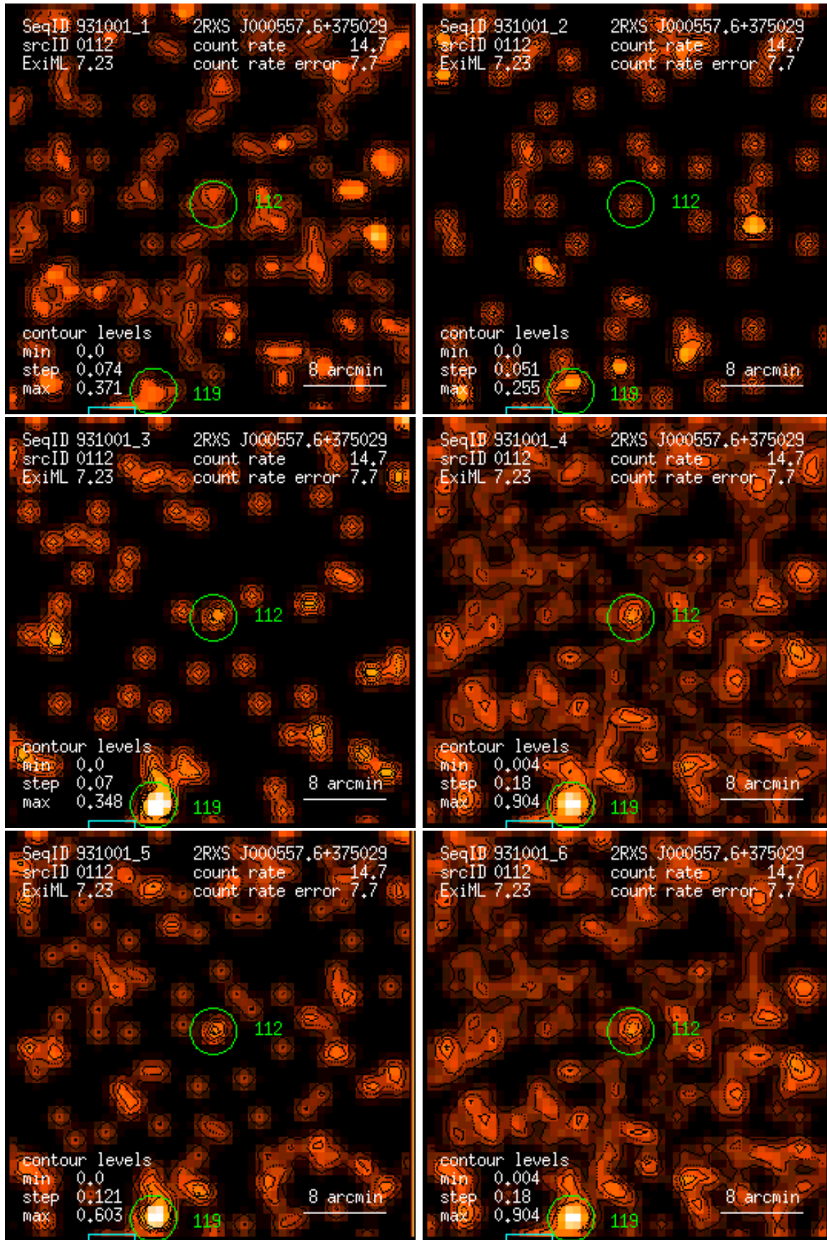
Figure 112: RASS 931001: detection 0112: band rate images, Gaussian filter: (1) PSPC channels 11 – 41, (2) 52 – 90, (3) 91 – 201, (4) 11 – 235, (5) 52 – 201, (6) 11 – 201. Broad band rates in counts/ks. Band rate contour levels in counts/ks/arcmin 2 .
