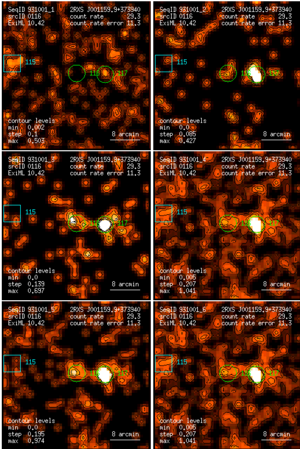
Figure 116: RASS 931001: detection 0116: band rate images, Gaussian filter: (1) PSPC channels 11 – 41, (2) 52 – 90, (3) 91 – 201, (4) 11 – 235, (5) 52 – 201, (6) 11 – 201. Broad band rates in counts/ks. Band rate contour levels in counts/ks/arcmin 2 .
