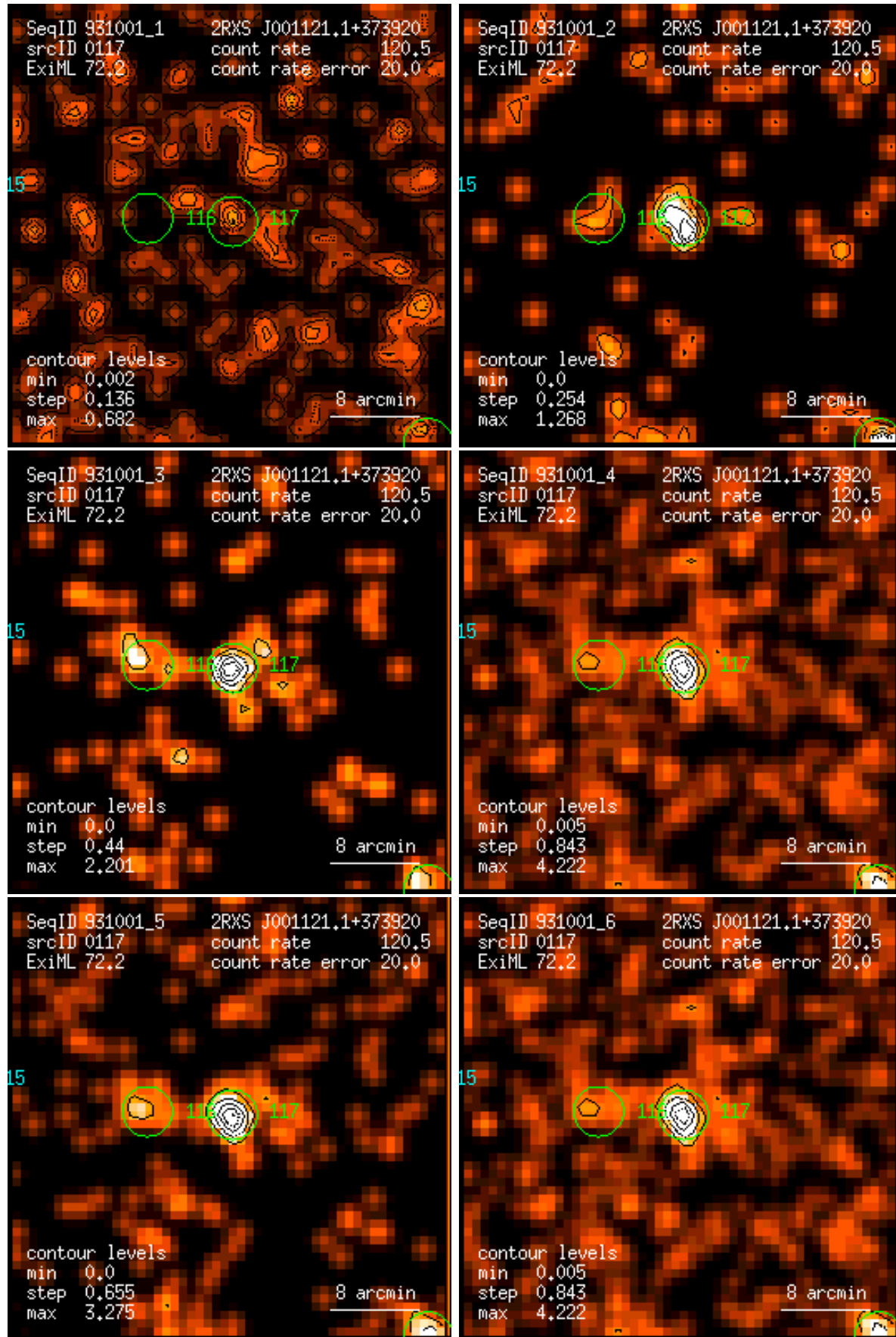
Figure 117: RASS 931001: detection 0117: band rate images, Gaussian filter: (1) PSPC channels 11 – 41, (2) 52 – 90, (3) 91 – 201, (4) 11 – 235, (5) 52 – 201, (6) 11 – 201. Broad band rates in counts/ks. Band rate contour levels in counts/ks/arcmin 2 .
