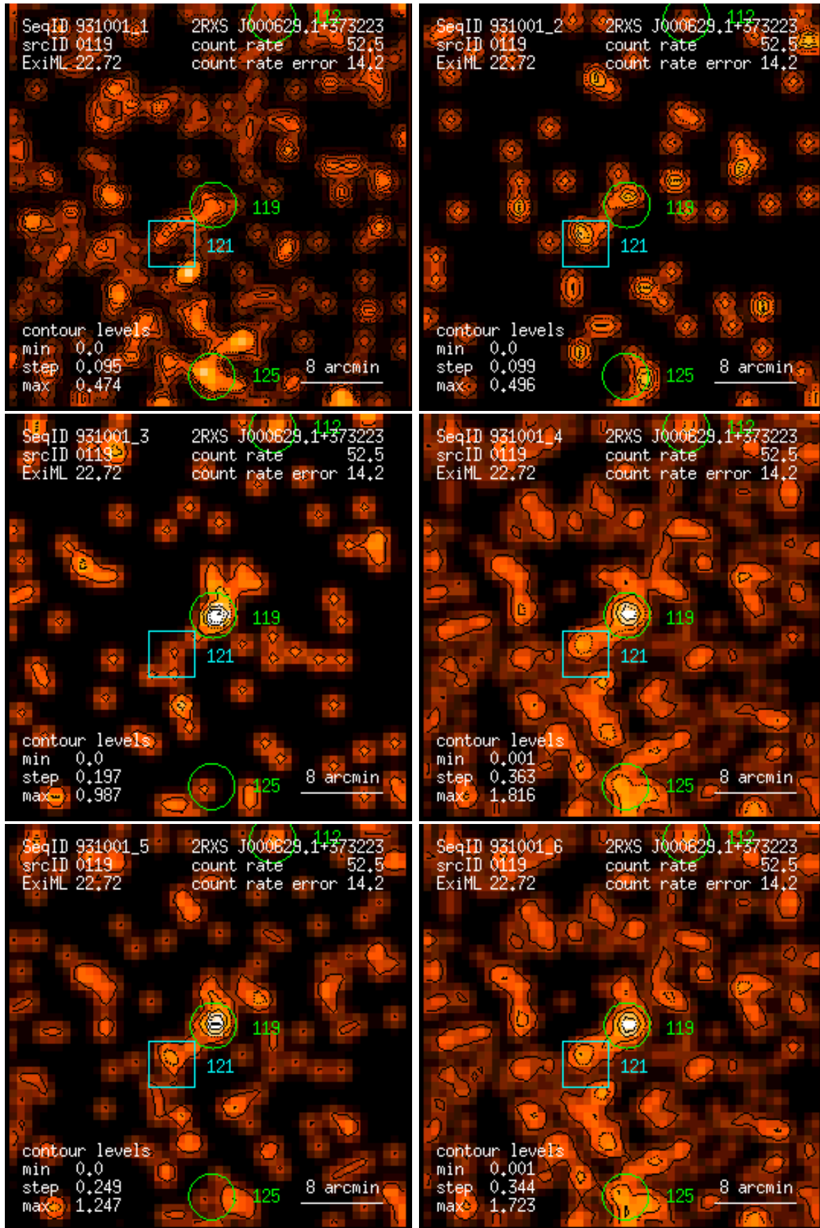
Figure 119: RASS 931001: detection 0119: band rate images, Gaussian filter: (1) PSPC channels 11 – 41, (2) 52 – 90, (3) 91 – 201, (4) 11 – 235, (5) 52 – 201, (6) 11 – 201. Broad band rates in counts/ks. Band rate contour levels in counts/ks/arcmin 2 .
