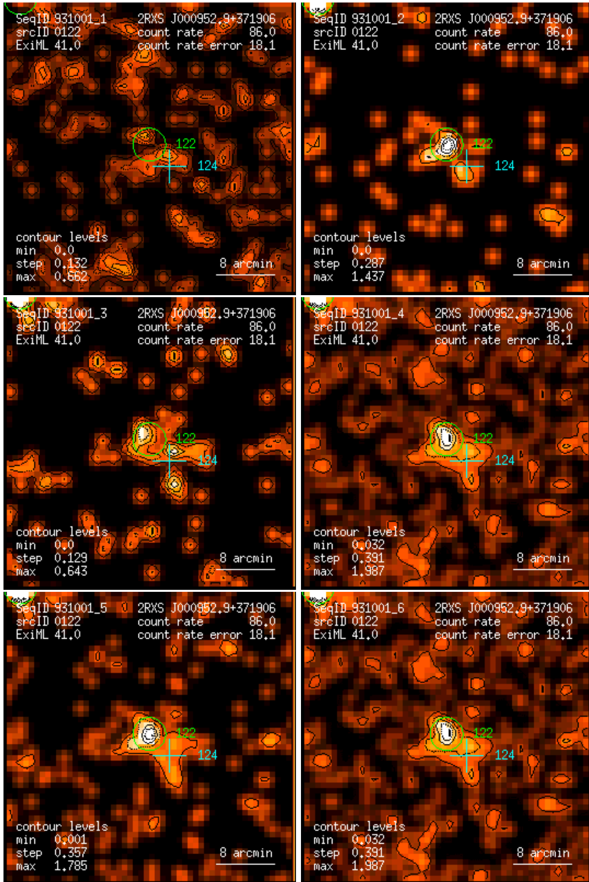
Figure 122: RASS 931001: detection 0122: band rate images, Gaussian filter: (1) PSPC channels 11 – 41, (2) 52 – 90, (3) 91 – 201, (4) 11 – 235, (5) 52 – 201, (6) 11 – 201. Broad band rates in counts/ks. Band rate contour levels in counts/ks/arcmin 2 .
