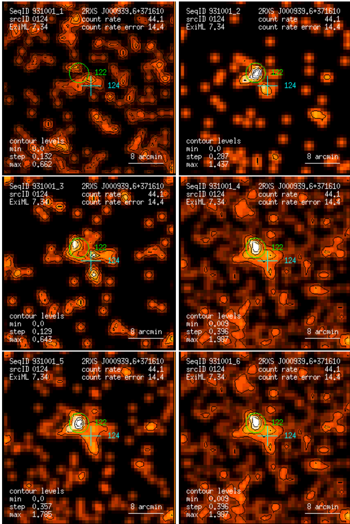
Figure 124: RASS 931001: detection 0124: band rate images, Gaussian filter: (1) PSPC channels 11 – 41, (2) 52 – 90, (3) 91 – 201, (4) 11 – 235, (5) 52 – 201, (6) 11 – 201. Broad band rates in counts/ks. Band rate contour levels in counts/ks/arcmin 2 .
