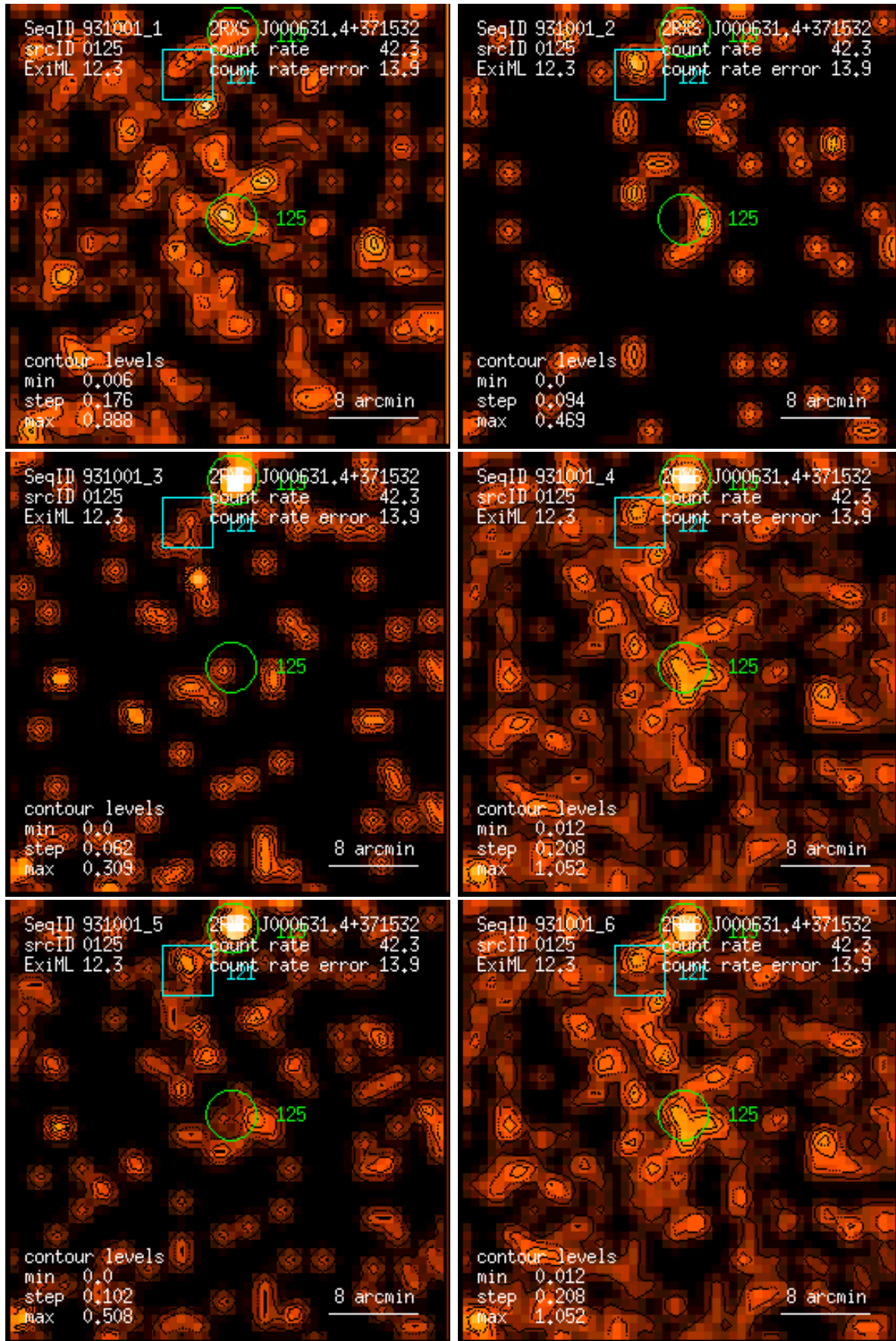
Figure 125: RASS 931001: detection 0125: band rate images, Gaussian filter: (1) PSPC channels 11 – 41, (2) 52 – 90, (3) 91 – 201, (4) 11 – 235, (5) 52 – 201, (6) 11 – 201. Broad band rates in counts/ks. Band rate contour levels in counts/ks/arcmin 2 .
