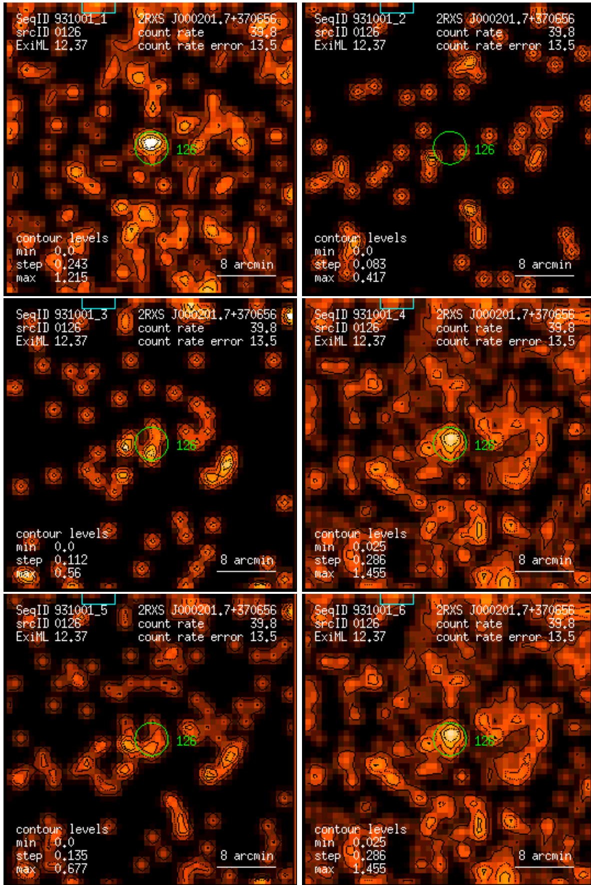
Figure 126: RASS 931001: detection 0126: band rate images, Gaussian filter: (1) PSPC channels 11 – 41, (2) 52 – 90, (3) 91 – 201, (4) 11 – 235, (5) 52 – 201, (6) 11 – 201. Broad band rates in counts/ks. Band rate contour levels in counts/ks/arcmin 2 .
