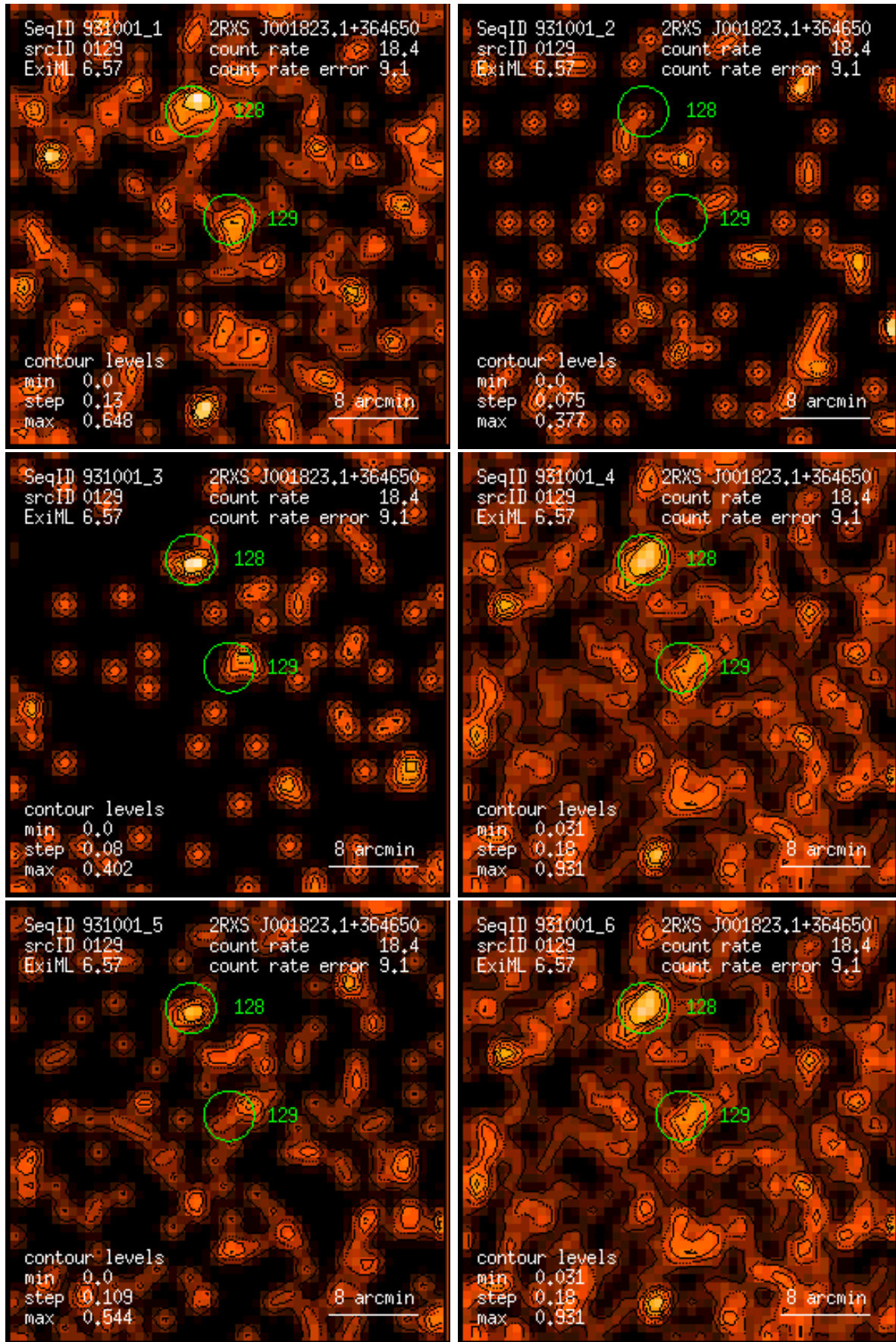
Figure 129: RASS 931001: detection 0129: band rate images, Gaussian filter: (1) PSPC channels 11 – 41, (2) 52 – 90, (3) 91 – 201, (4) 11 – 235, (5) 52 – 201, (6) 11 – 201. Broad band rates in counts/ks. Band rate contour levels in counts/ks/arcmin 2 .
