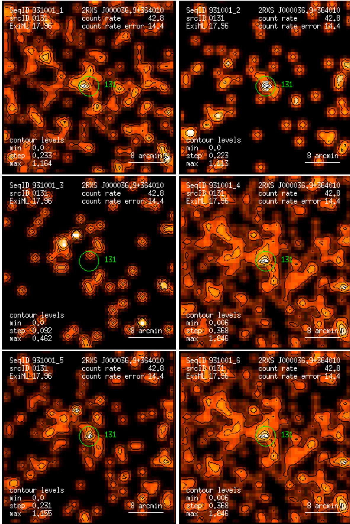
Figure 131: RASS 931001: detection 0131: band rate images, Gaussian filter: (1) PSPC channels 11 – 41, (2) 52 – 90, (3) 91 – 201, (4) 11 – 235, (5) 52 – 201, (6) 11 – 201. Broad band rates in counts/ks. Band rate contour levels in counts/ks/arcmin 2 .
