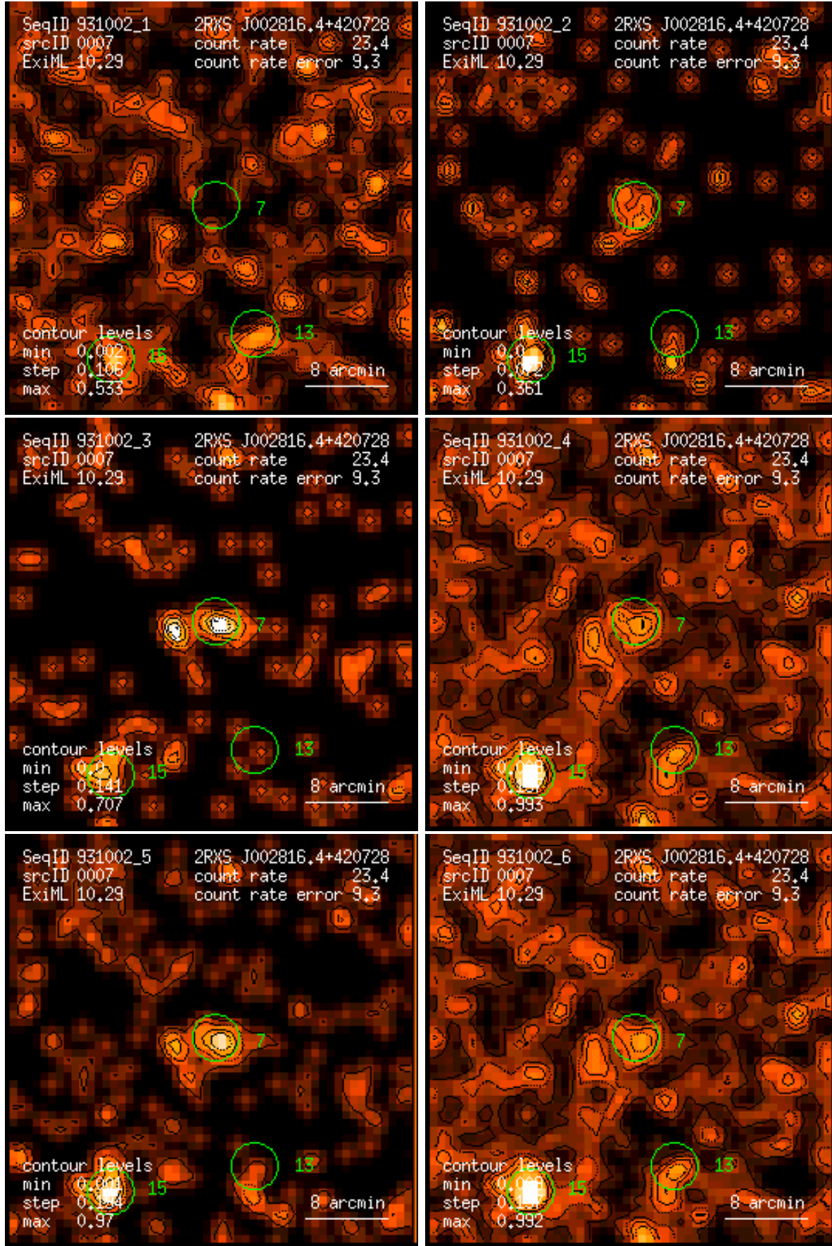
Figure 7: RASS 931002: detection 0007: band rate images, Gaussian filter: (1) PSPC channels 11 – 41, (2) 52 – 90, (3) 91 – 201, (4) 11 – 235, (5) 52 – 201, (6) 11 – 201. Broad band rates in counts/ks. Band rate contour levels in counts/ks/arcmin 2 .
