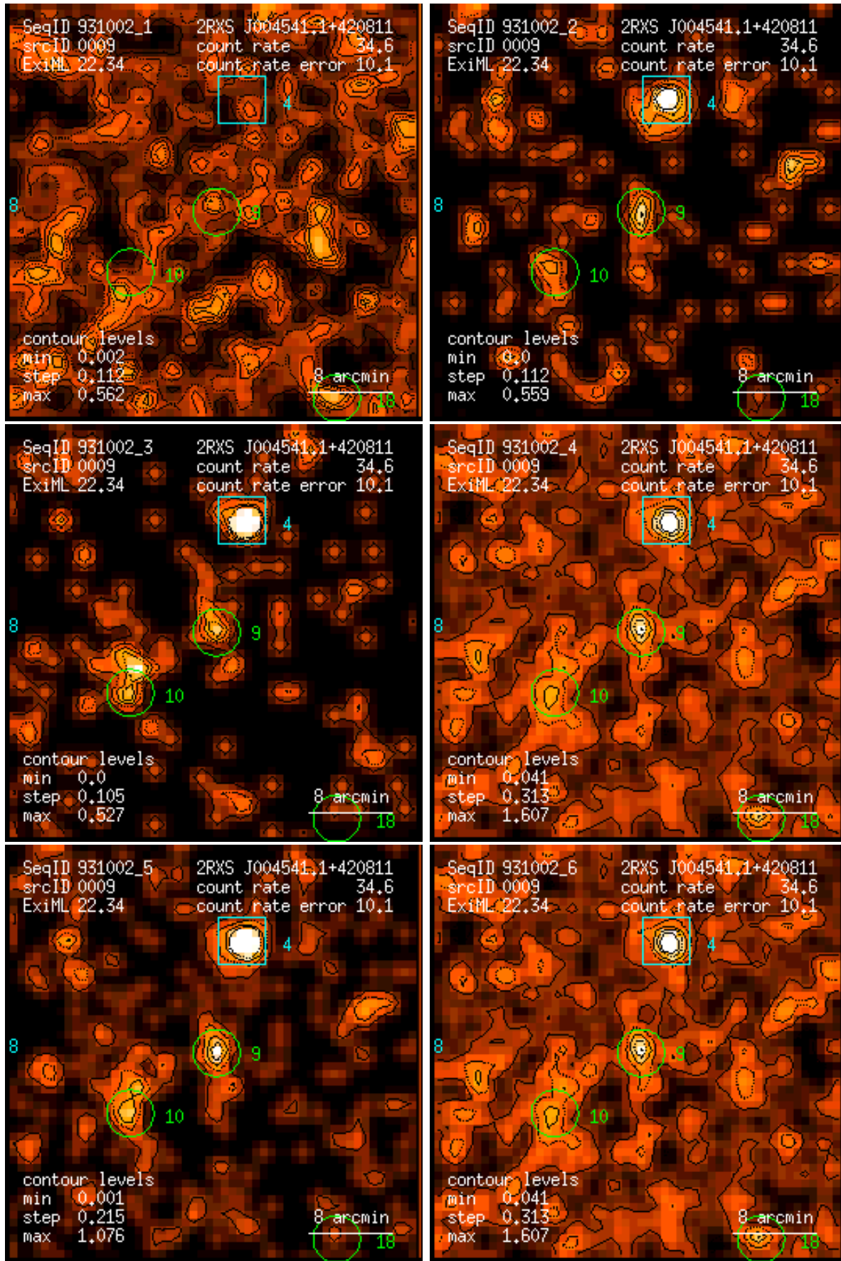
Figure 9: RASS 931002: detection 0009: band rate images, Gaussian filter: (1) PSPC channels 11 – 41, (2) 52 – 90, (3) 91 – 201, (4) 11 – 235, (5) 52 – 201, (6) 11 – 201. Broad band rates in counts/ks. Band rate contour levels in counts/ks/arcmin 2 .
