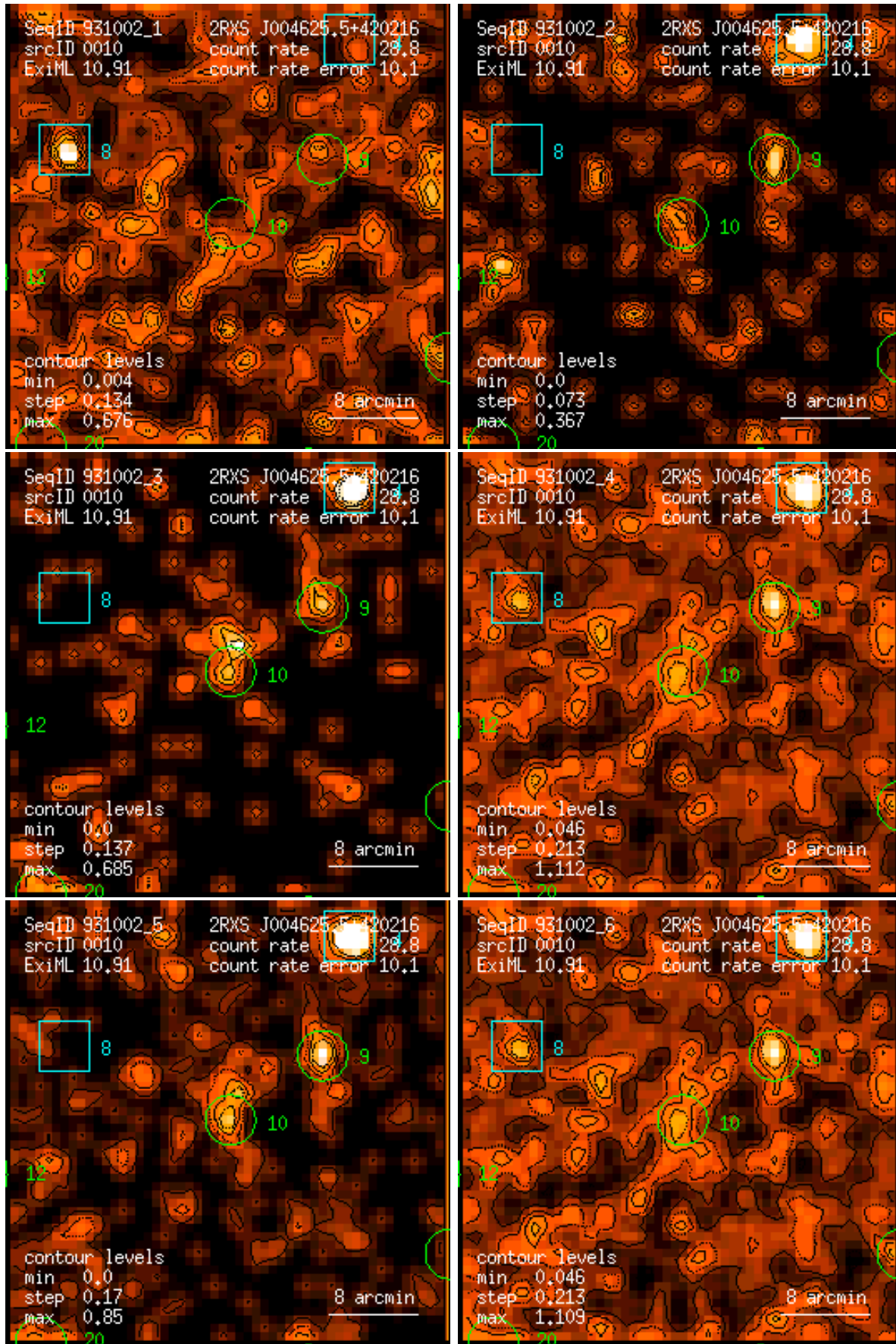
Figure 10: RASS 931002: detection 0010: band rate images, Gaussian filter: (1) PSPC channels 11 – 41, (2) 52 – 90, (3) 91 – 201, (4) 11 – 235, (5) 52 – 201, (6) 11 – 201. Broad band rates in counts/ks. Band rate contour levels in counts/ks/arcmin 2 .
