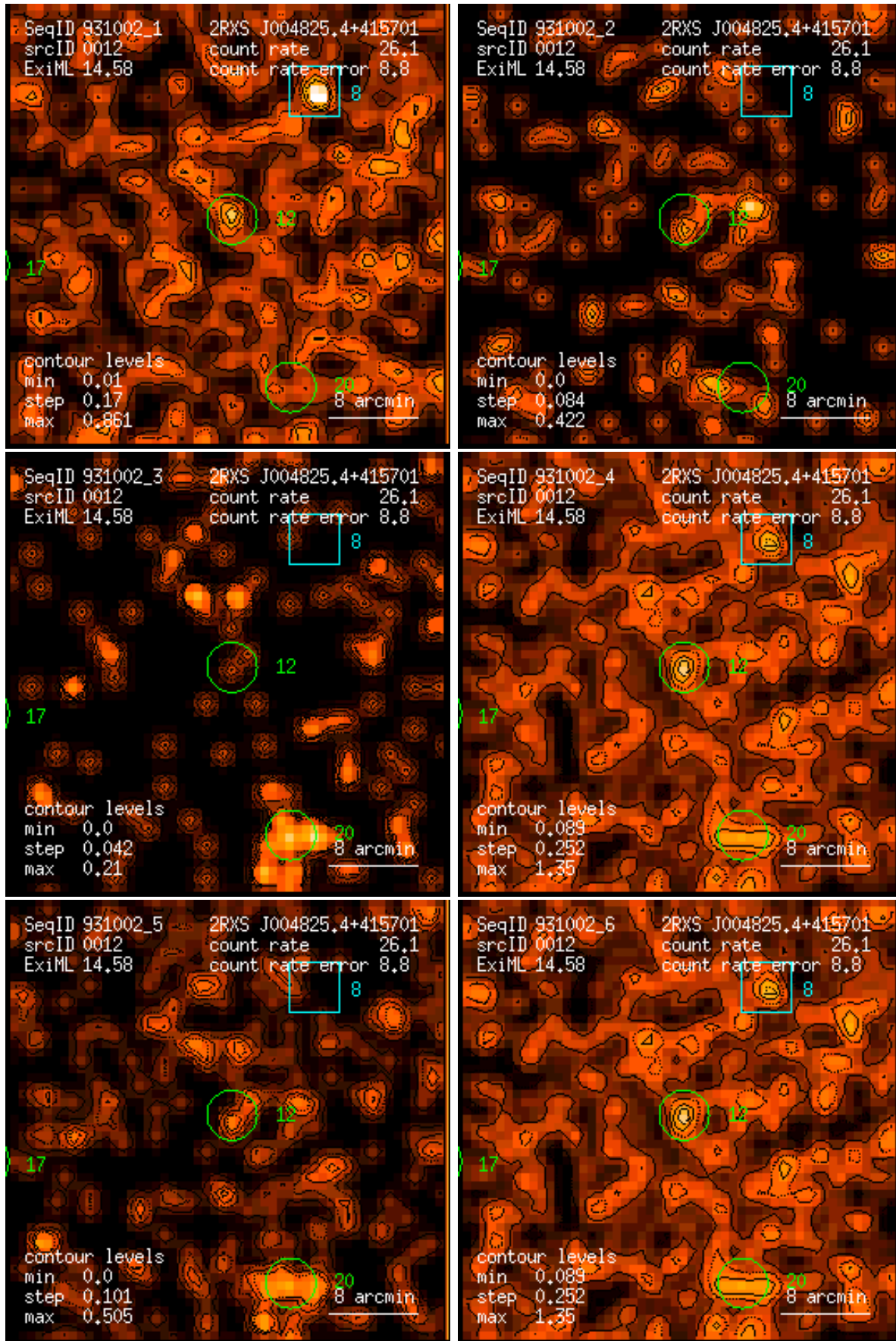
Figure 12: RASS 931002: detection 0012: band rate images, Gaussian filter: (1) PSPC channels 11 – 41, (2) 52 – 90, (3) 91 – 201, (4) 11 – 235, (5) 52 – 201, (6) 11 – 201. Broad band rates in counts/ks. Band rate contour levels in counts/ks/arcmin 2 .
