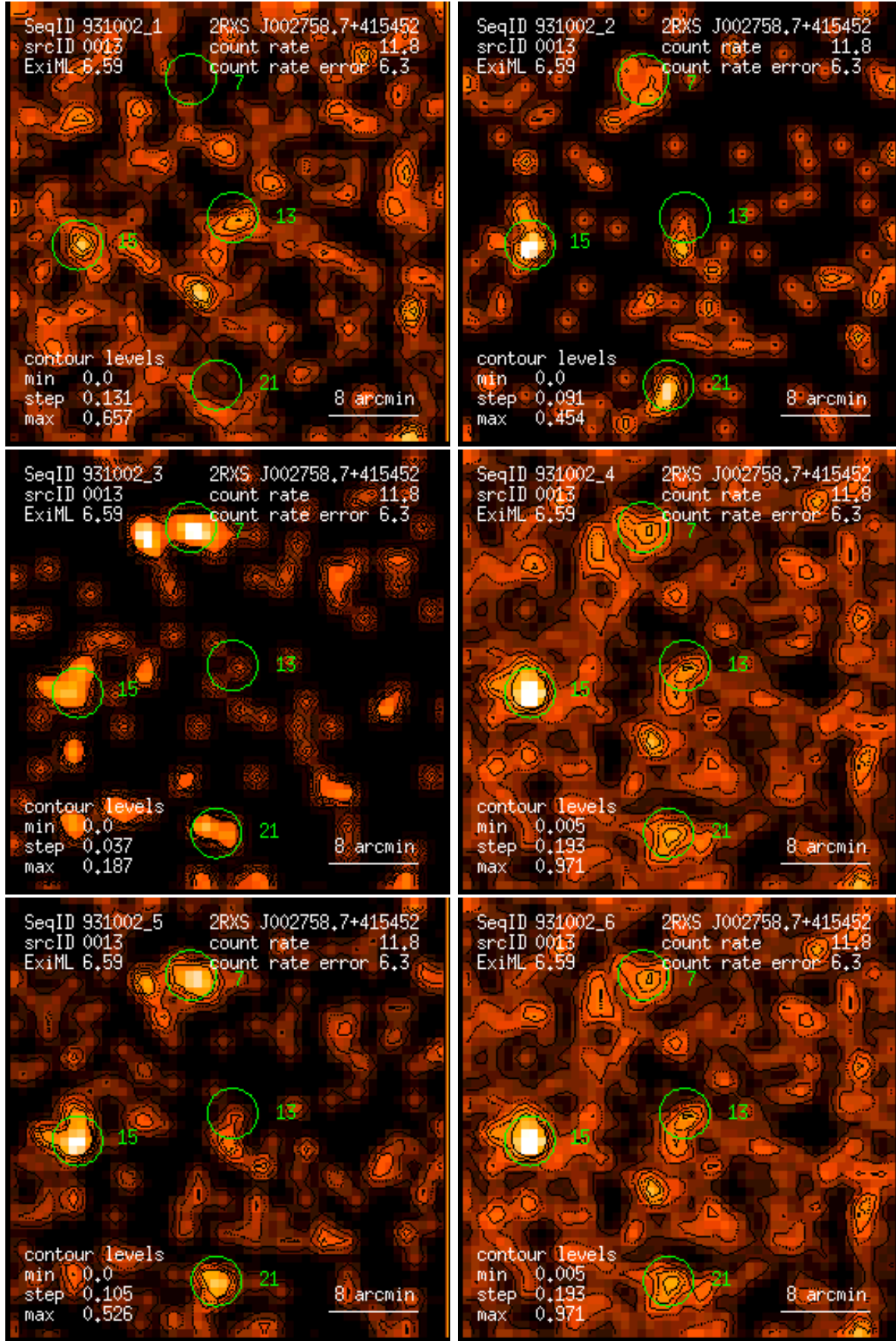
Figure 13: RASS 931002: detection 0013: band rate images, Gaussian filter: (1) PSPC channels 11 – 41, (2) 52 – 90, (3) 91 – 201, (4) 11 – 235, (5) 52 – 201, (6) 11 – 201. Broad band rates in counts/ks. Band rate contour levels in counts/ks/arcmin 2 .
