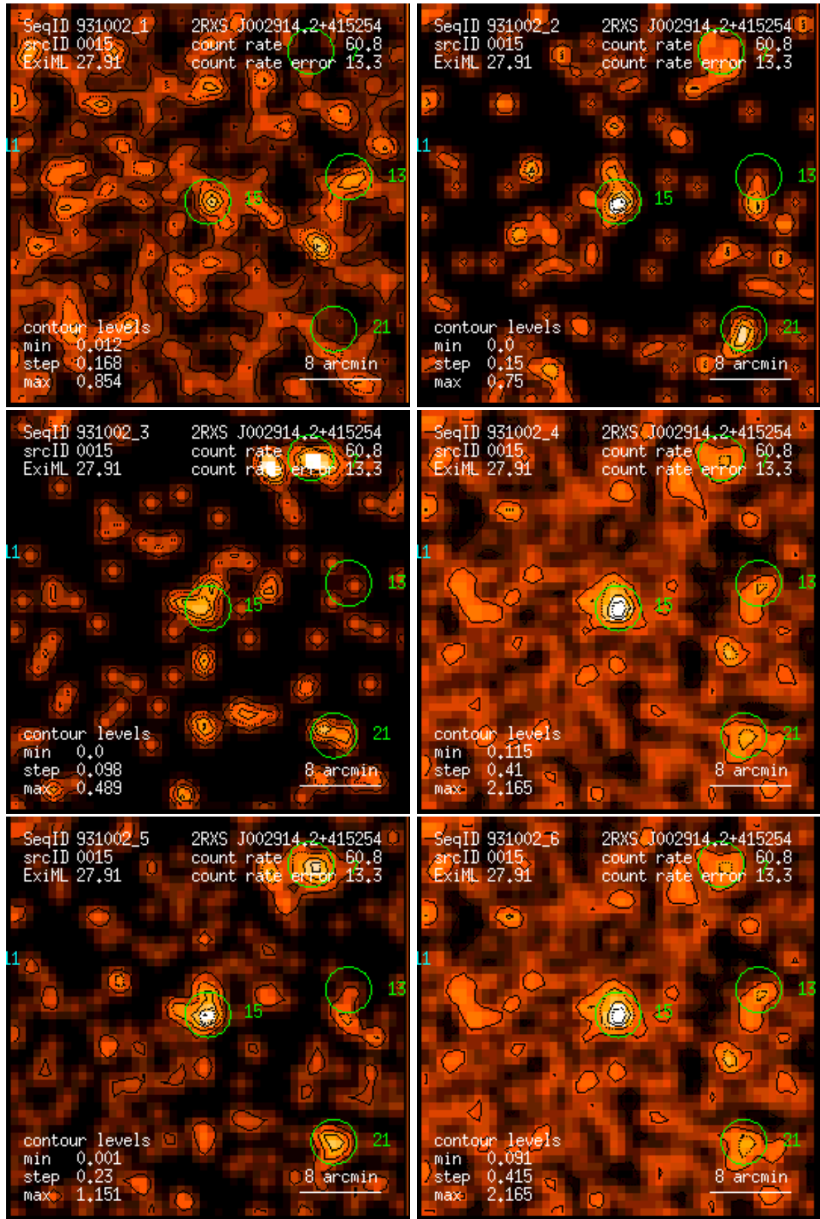
Figure 15: RASS 931002: detection 0015: band rate images, Gaussian filter: (1) PSPC channels 11 – 41, (2) 52 – 90, (3) 91 – 201, (4) 11 – 235, (5) 52 – 201, (6) 11 – 201. Broad band rates in counts/ks. Band rate contour levels in counts/ks/arcmin 2 .
