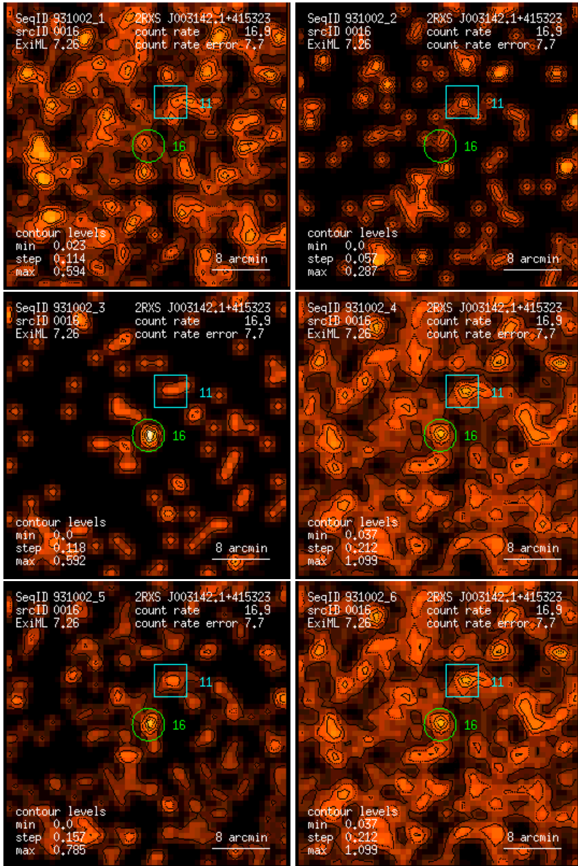
Figure 16: RASS 931002: detection 0016: band rate images, Gaussian filter: (1) PSPC channels 11 – 41, (2) 52 – 90, (3) 91 – 201, (4) 11 – 235, (5) 52 – 201, (6) 11 – 201. Broad band rates in counts/ks. Band rate contour levels in counts/ks/arcmin 2 .
