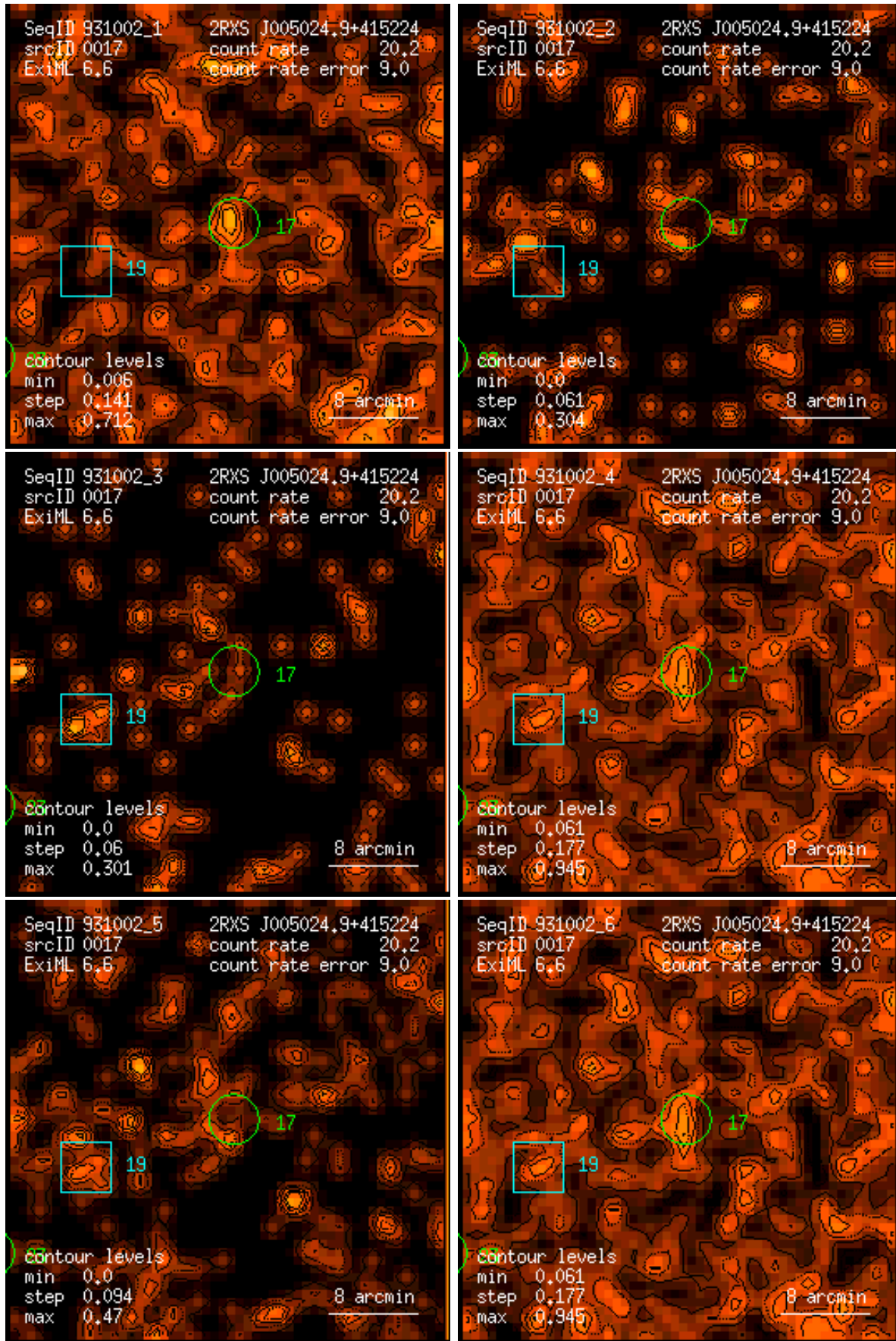
Figure 17: RASS 931002: detection 0017: band rate images, Gaussian filter: (1) PSPC channels 11 – 41, (2) 52 – 90, (3) 91 – 201, (4) 11 – 235, (5) 52 – 201, (6) 11 – 201. Broad band rates in counts/ks. Band rate contour levels in counts/ks/arcmin 2 .
