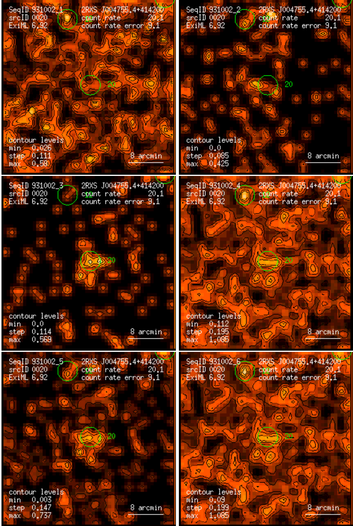
Figure 20: RASS 931002: detection 0020: band rate images, Gaussian filter: (1) PSPC channels 11 – 41, (2) 52 – 90, (3) 91 – 201, (4) 11 – 235, (5) 52 – 201, (6) 11 – 201. Broad band rates in counts/ks. Band rate contour levels in counts/ks/arcmin 2 .
