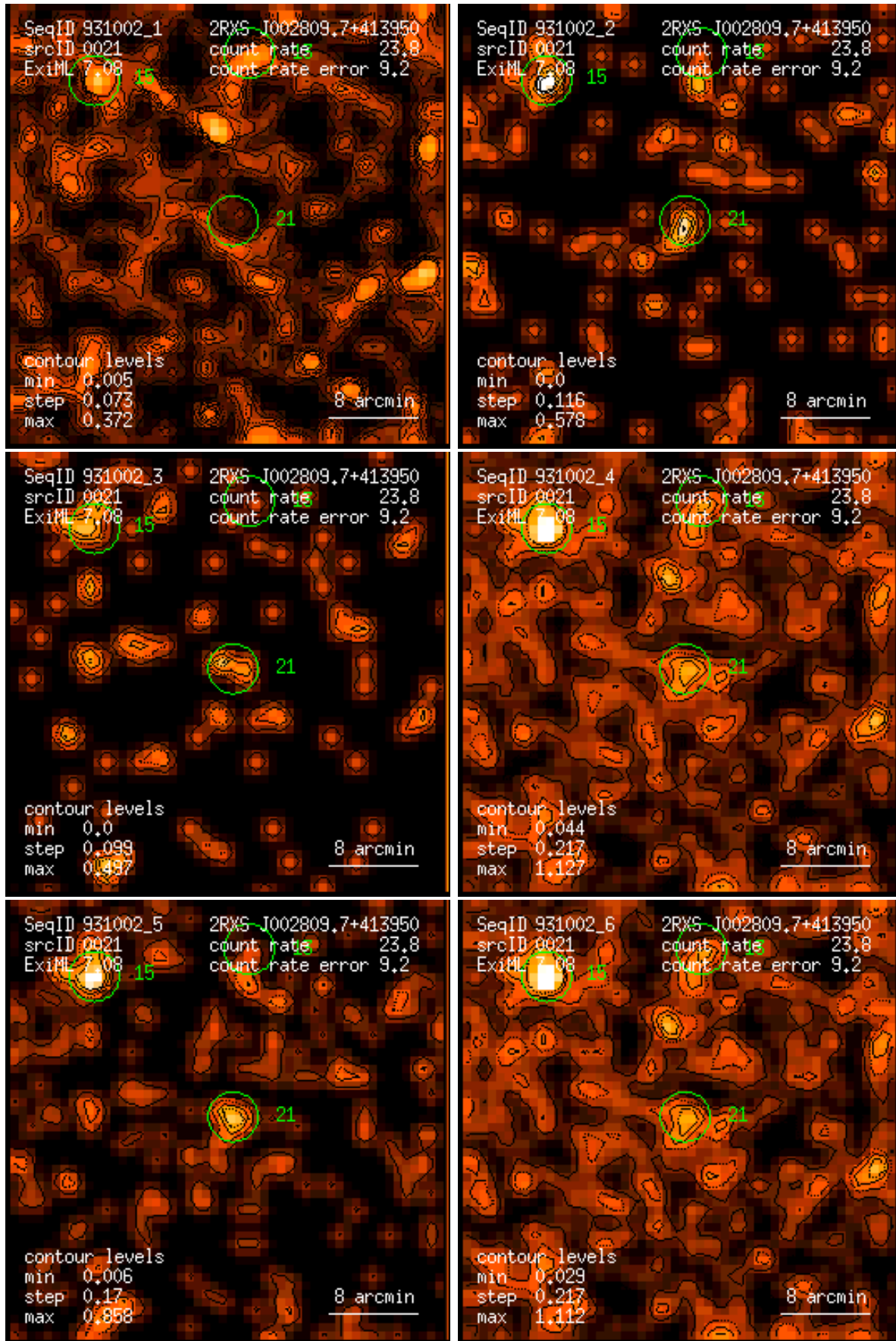
Figure 21: RASS 931002: detection 0021: band rate images, Gaussian filter: (1) PSPC channels 11 – 41, (2) 52 – 90, (3) 91 – 201, (4) 11 – 235, (5) 52 – 201, (6) 11 – 201. Broad band rates in counts/ks. Band rate contour levels in counts/ks/arcmin 2 .
