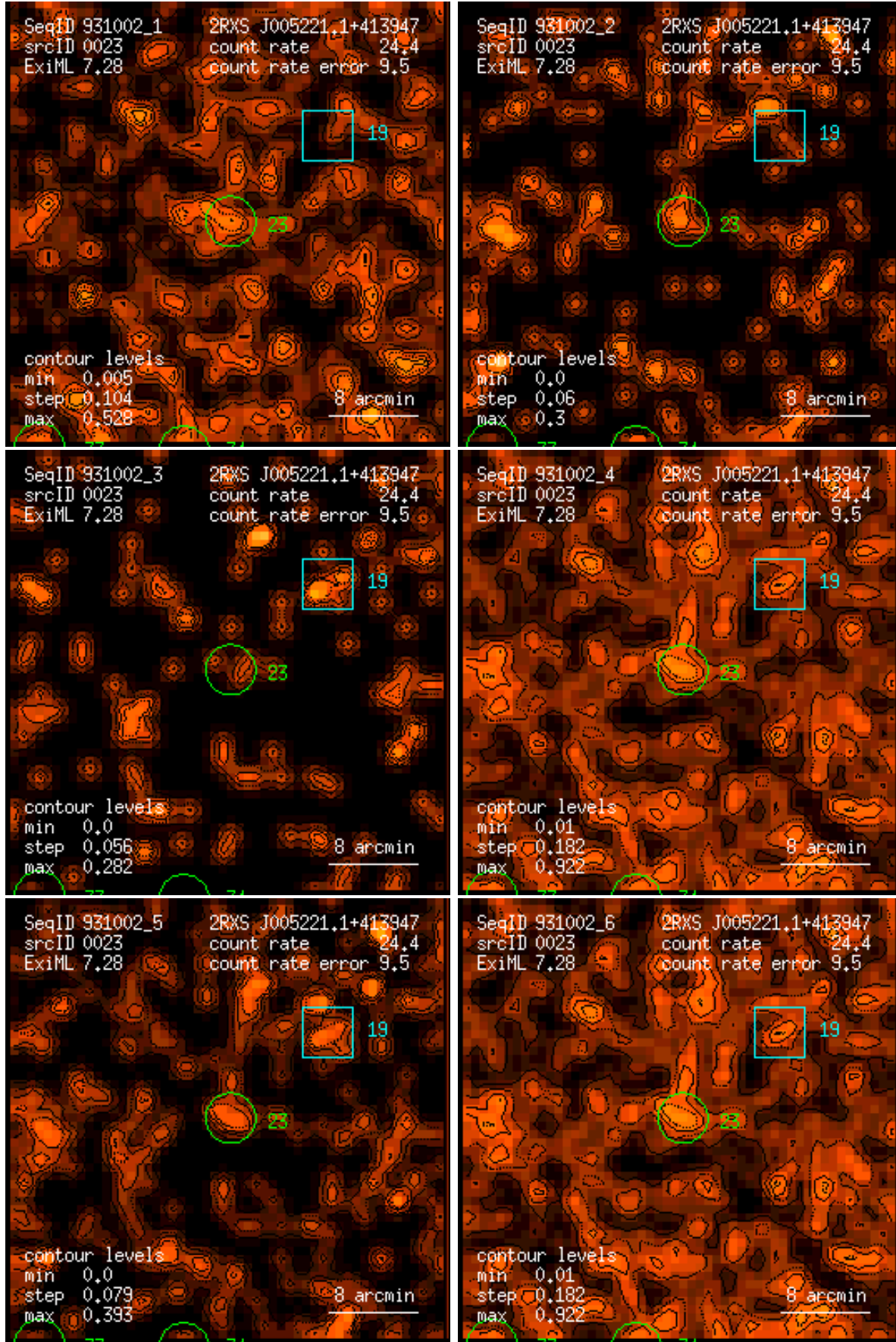
Figure 23: RASS 931002: detection 0023: band rate images, Gaussian filter: (1) PSPC channels 11 – 41, (2) 52 – 90, (3) 91 – 201, (4) 11 – 235, (5) 52 – 201, (6) 11 – 201. Broad band rates in counts/ks. Band rate contour levels in counts/ks/arcmin 2 .
