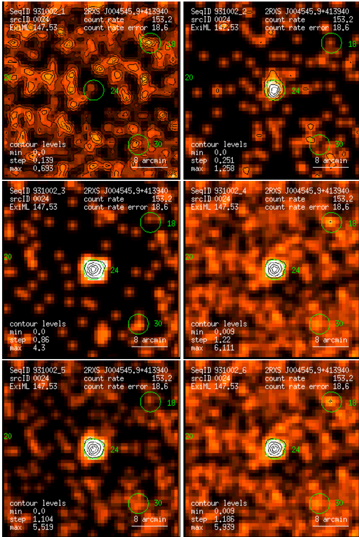
Figure 24: RASS 931002: detection 0024: band rate images, Gaussian filter: (1) PSPC channels 11 – 41, (2) 52 – 90, (3) 91 – 201, (4) 11 – 235, (5) 52 – 201, (6) 11 – 201. Broad band rates in counts/ks. Band rate contour levels in counts/ks/arcmin 2 .
