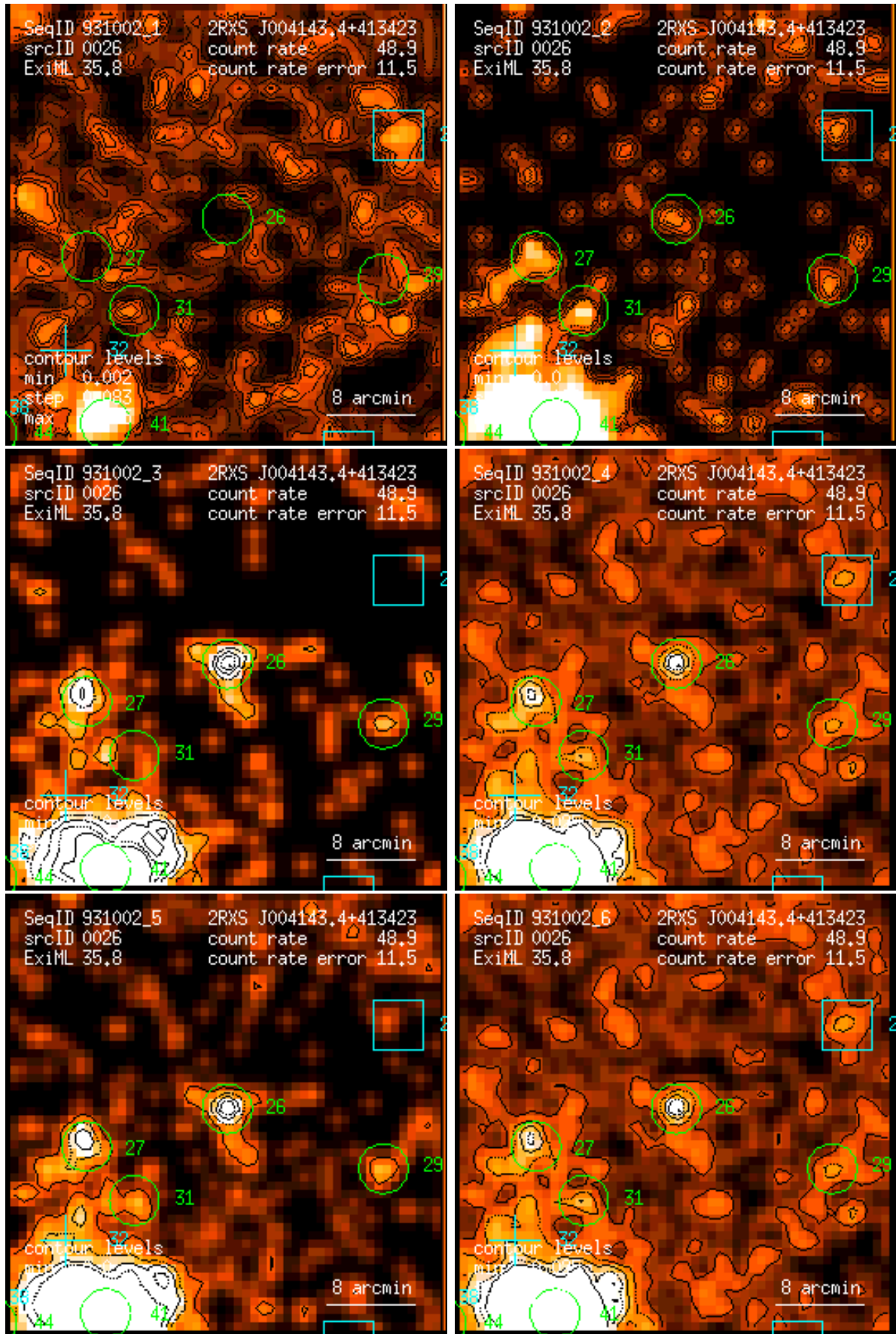
Figure 26: RASS 931002: detection 0026: band rate images, Gaussian filter: (1) PSPC channels 11 – 41, (2) 52 – 90, (3) 91 – 201, (4) 11 – 235, (5) 52 – 201, (6) 11 – 201. Broad band rates in counts/ks. Band rate contour levels in counts/ks/arcmin 2 .
