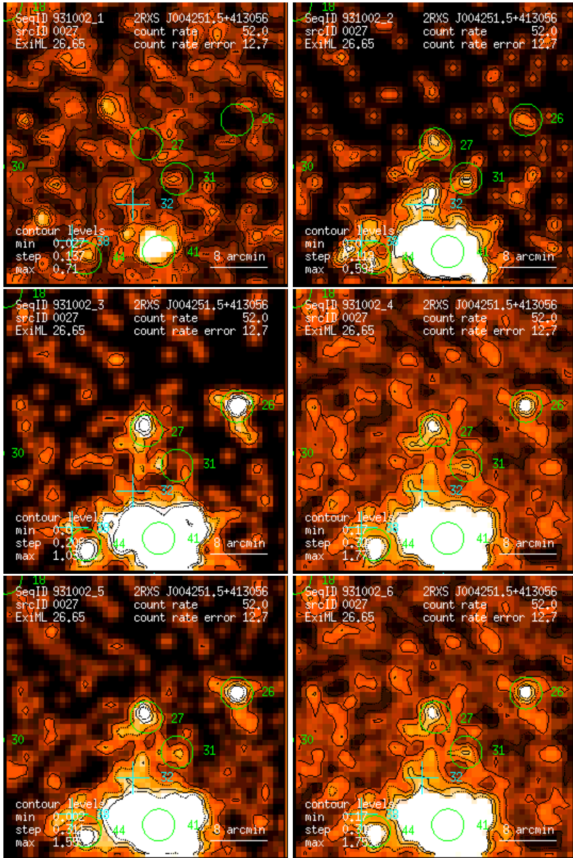
Figure 27: RASS 931002: detection 0027: band rate images, Gaussian filter: (1) PSPC channels 11 – 41, (2) 52 – 90, (3) 91 – 201, (4) 11 – 235, (5) 52 – 201, (6) 11 – 201. Broad band rates in counts/ks. Band rate contour levels in counts/ks/arcmin 2 .
