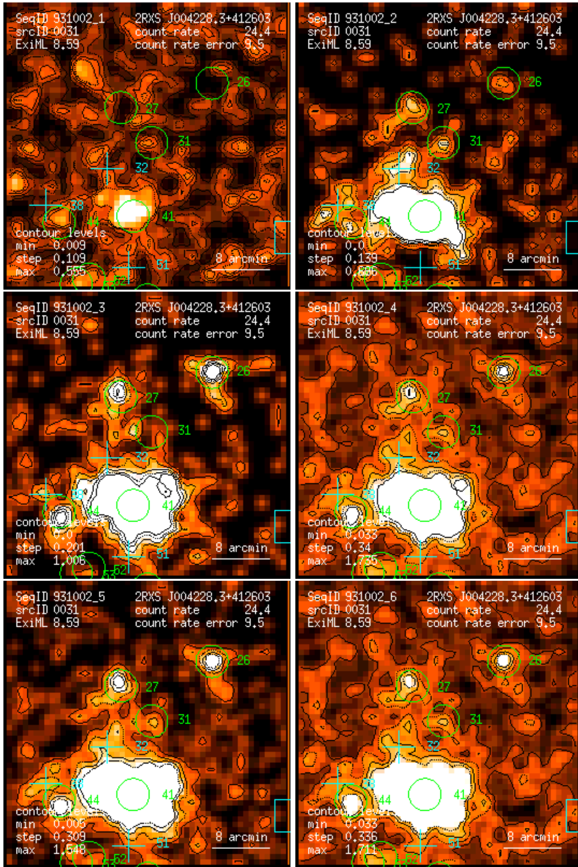
Figure 31: RASS 931002: detection 0031: band rate images, Gaussian filter: (1) PSPC channels 11 – 41, (2) 52 – 90, (3) 91 – 201, (4) 11 – 235, (5) 52 – 201, (6) 11 – 201. Broad band rates in counts/ks. Band rate contour levels in counts/ks/arcmin 2 .
