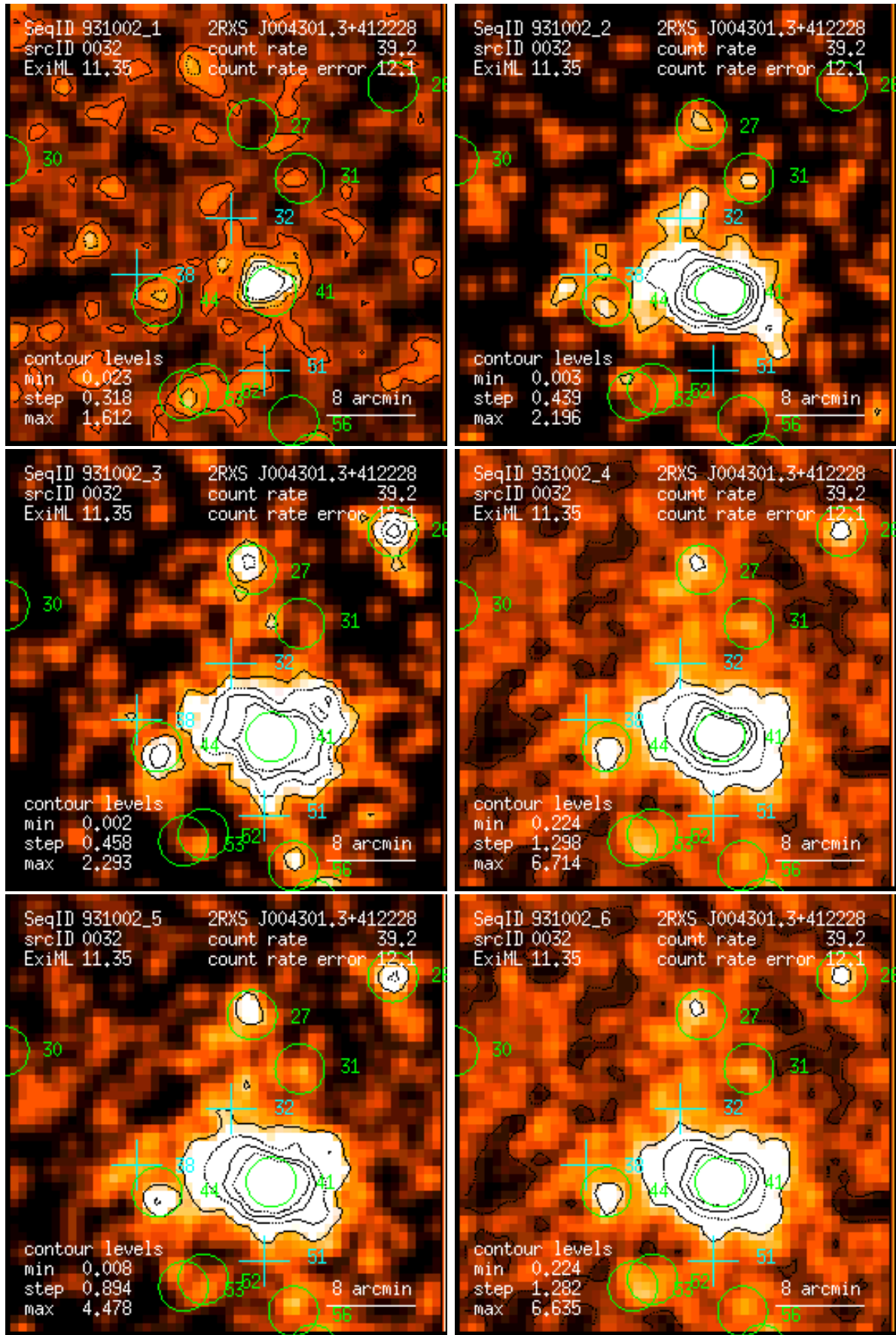
Figure 32: RASS 931002: detection 0032: band rate images, Gaussian filter: (1) PSPC channels 11 – 41, (2) 52 – 90, (3) 91 – 201, (4) 11 – 235, (5) 52 – 201, (6) 11 – 201. Broad band rates in counts/ks. Band rate contour levels in counts/ks/arcmin 2 .
