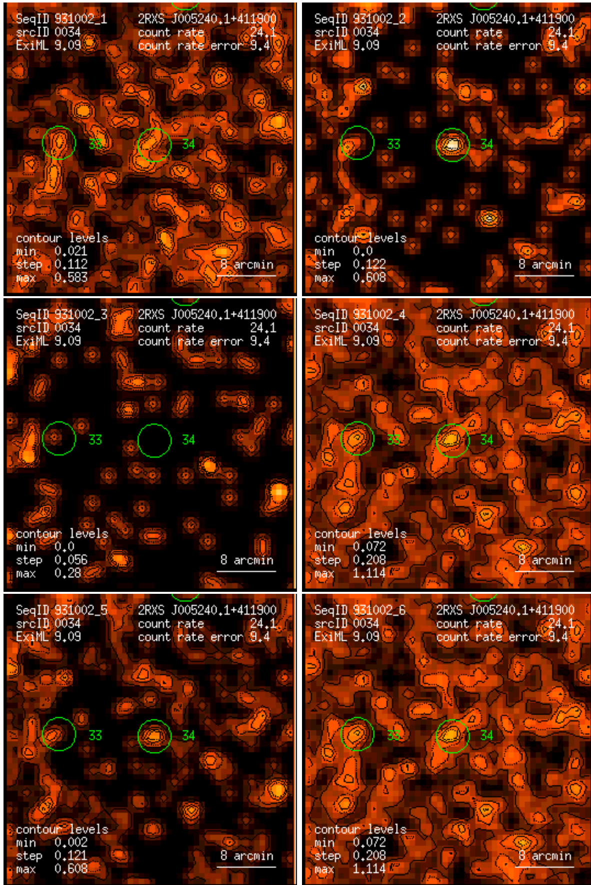
Figure 34: RASS 931002: detection 0034: band rate images, Gaussian filter: (1) PSPC channels 11 – 41, (2) 52 – 90, (3) 91 – 201, (4) 11 – 235, (5) 52 – 201, (6) 11 – 201. Broad band rates in counts/ks. Band rate contour levels in counts/ks/arcmin 2 .
