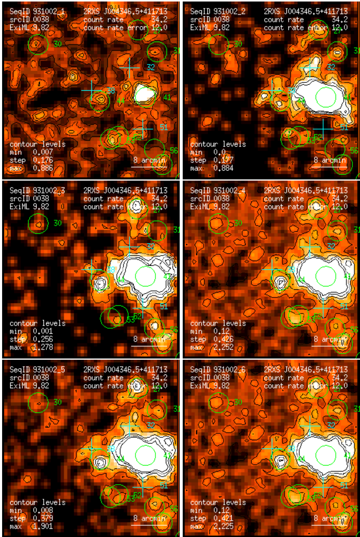
Figure 38: RASS 931002: detection 0038: band rate images, Gaussian filter: (1) PSPC channels 11 – 41, (2) 52 – 90, (3) 91 – 201, (4) 11 – 235, (5) 52 – 201, (6) 11 – 201. Broad band rates in counts/ks. Band rate contour levels in counts/ks/arcmin 2 .
