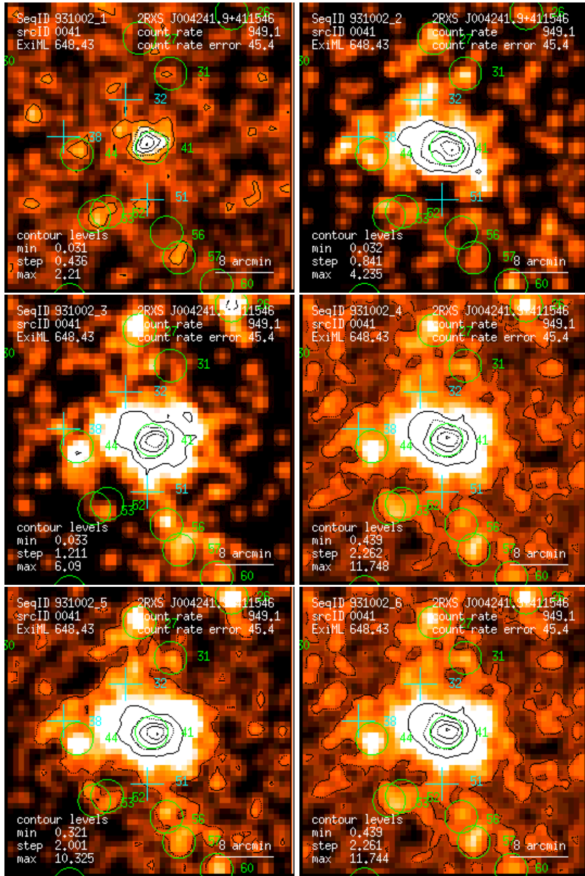
Figure 41: RASS 931002: detection 0041: band rate images, Gaussian filter: (1) PSPC channels 11 – 41, (2) 52 – 90, (3) 91 – 201, (4) 11 – 235, (5) 52 – 201, (6) 11 – 201. Broad band rates in counts/ks. Band rate contour levels in counts/ks/arcmin 2 .
