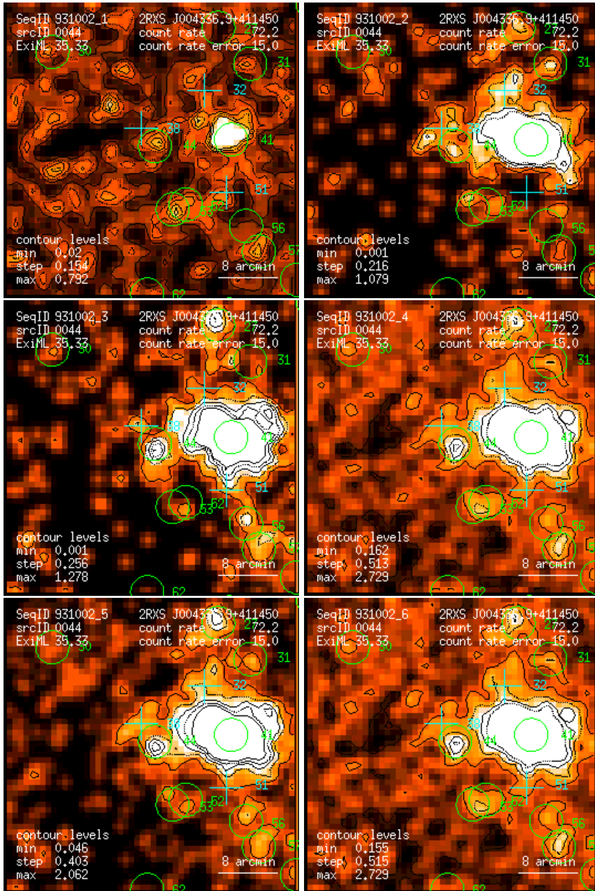
Figure 44: RASS 931002: detection 0044: band rate images, Gaussian filter: (1) PSPC channels 11 – 41, (2) 52 – 90, (3) 91 – 201, (4) 11 – 235, (5) 52 – 201, (6) 11 – 201. Broad band rates in counts/ks. Band rate contour levels in counts/ks/arcmin 2 .
