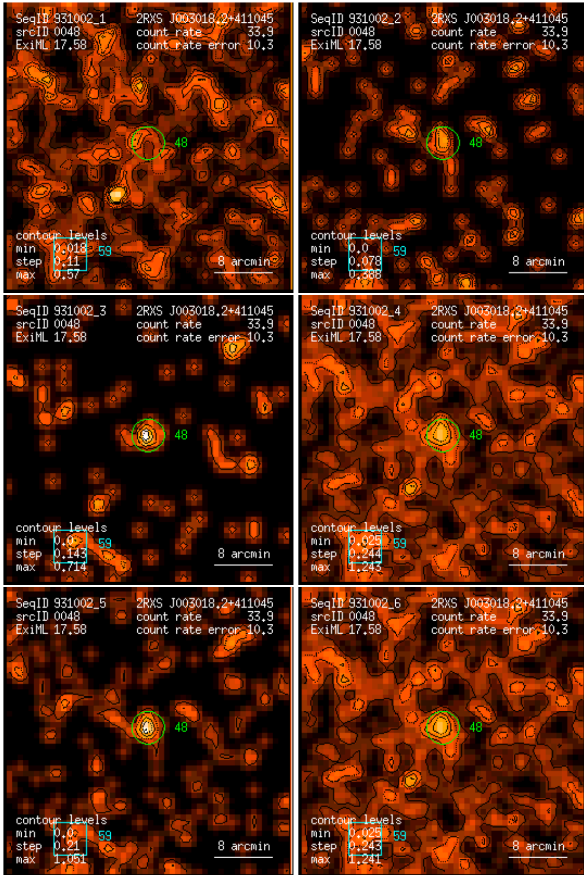
Figure 48: RASS 931002: detection 0048: band rate images, Gaussian filter: (1) PSPC channels 11 – 41, (2) 52 – 90, (3) 91 – 201, (4) 11 – 235, (5) 52 – 201, (6) 11 – 201. Broad band rates in counts/ks. Band rate contour levels in counts/ks/arcmin 2 .
