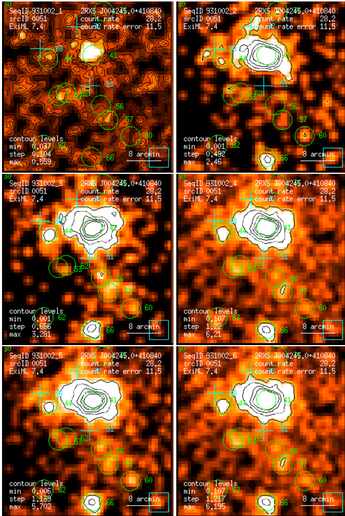
Figure 51: RASS 931002: detection 0051: band rate images, Gaussian filter: (1) PSPC channels 11 – 41, (2) 52 – 90, (3) 91 – 201, (4) 11 – 235, (5) 52 – 201, (6) 11 – 201. Broad band rates in counts/ks. Band rate contour levels in counts/ks/arcmin 2 .
