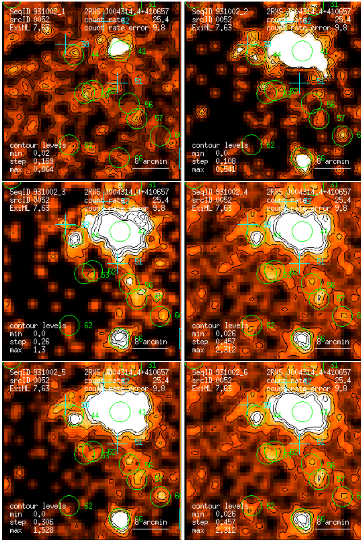
Figure 52: RASS 931002: detection 0052: band rate images, Gaussian filter: (1) PSPC channels 11 – 41, (2) 52 – 90, (3) 91 – 201, (4) 11 – 235, (5) 52 – 201, (6) 11 – 201. Broad band rates in counts/ks. Band rate contour levels in counts/ks/arcmin 2 .
