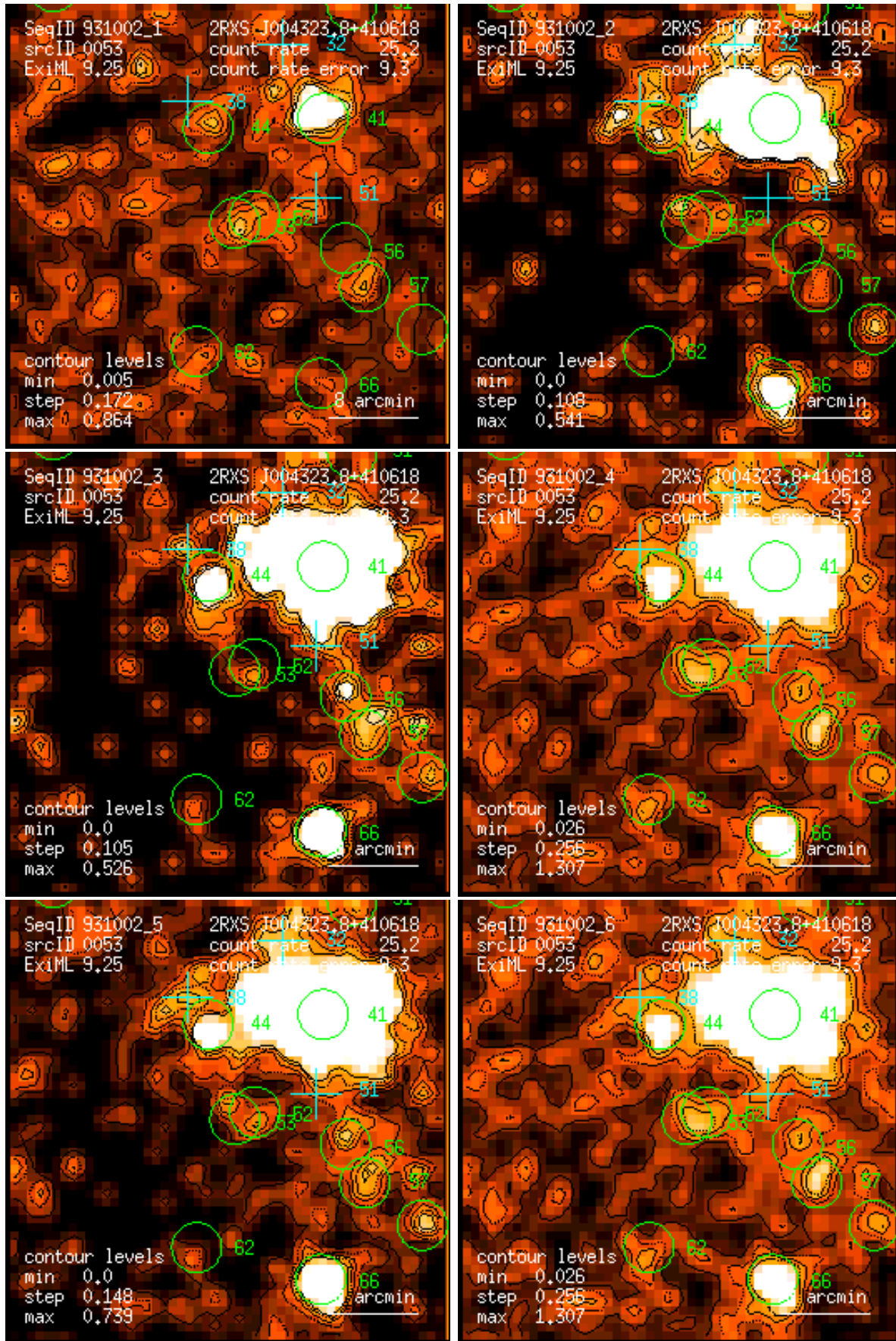
Figure 53: RASS 931002: detection 0053: band rate images, Gaussian filter: (1) PSPC channels 11 – 41, (2) 52 – 90, (3) 91 – 201, (4) 11 – 235, (5) 52 – 201, (6) 11 – 201. Broad band rates in counts/ks. Band rate contour levels in counts/ks/arcmin 2 .
