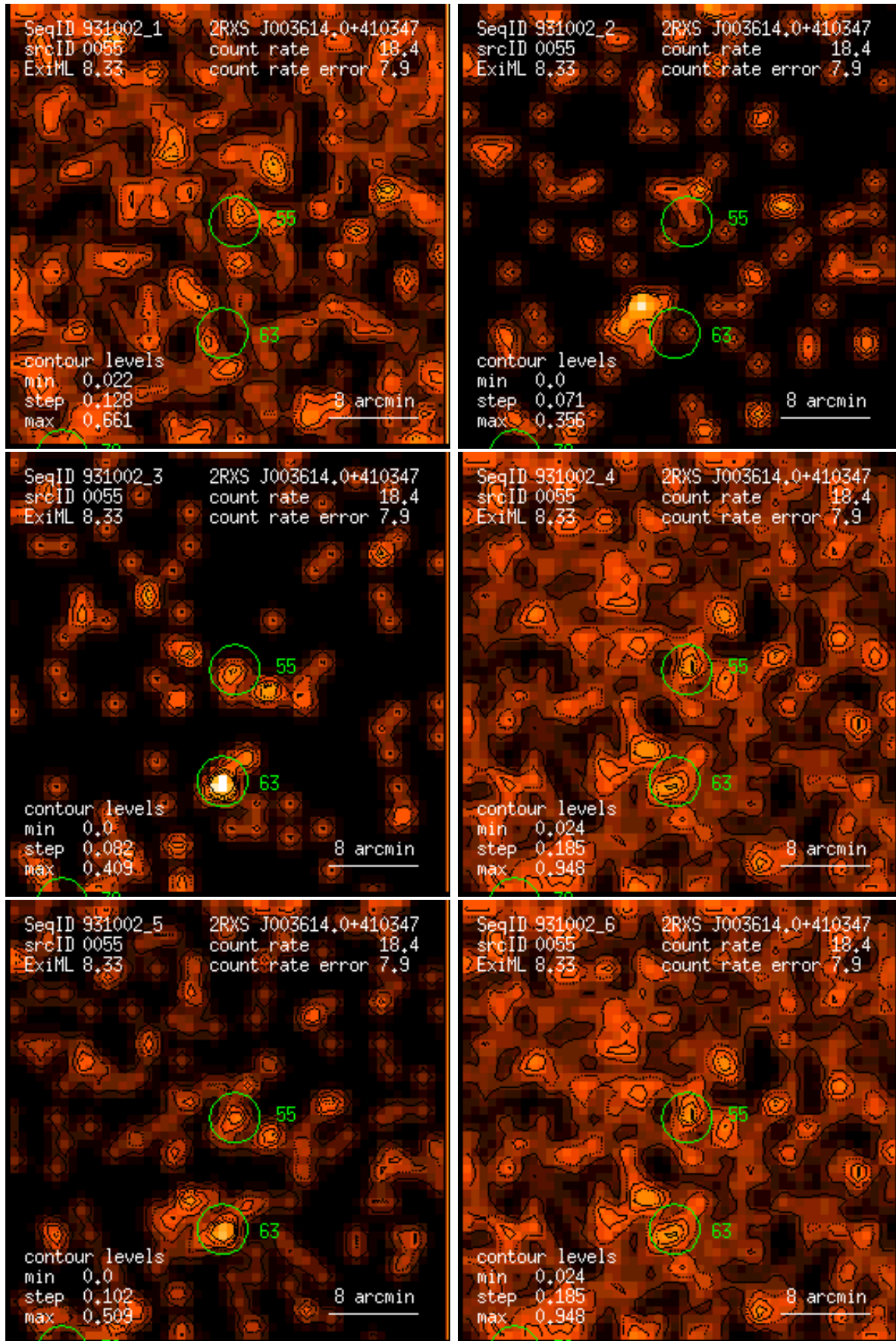
Figure 55: RASS 931002: detection 0055: band rate images, Gaussian filter: (1) PSPC channels 11 – 41, (2) 52 – 90, (3) 91 – 201, (4) 11 – 235, (5) 52 – 201, (6) 11 – 201. Broad band rates in counts/ks. Band rate contour levels in counts/ks/arcmin 2 .
