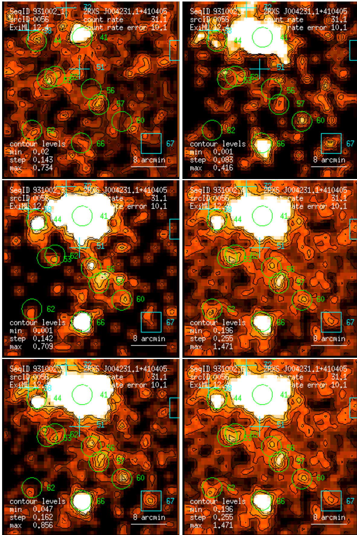
Figure 56: RASS 931002: detection 0056: band rate images, Gaussian filter: (1) PSPC channels 11 – 41, (2) 52 – 90, (3) 91 – 201, (4) 11 – 235, (5) 52 – 201, (6) 11 – 201. Broad band rates in counts/ks. Band rate contour levels in counts/ks/arcmin 2 .
