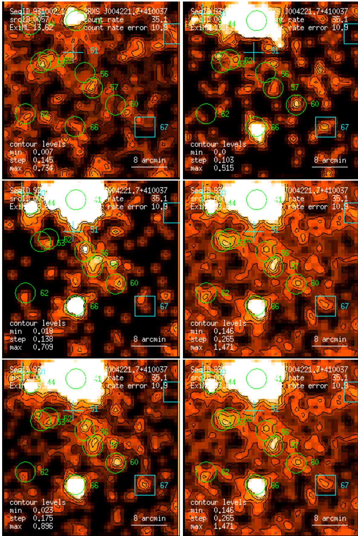
Figure 57: RASS 931002: detection 0057: band rate images, Gaussian filter: (1) PSPC channels 11 – 41, (2) 52 – 90, (3) 91 – 201, (4) 11 – 235, (5) 52 – 201, (6) 11 – 201. Broad band rates in counts/ks. Band rate contour levels in counts/ks/arcmin 2 .
