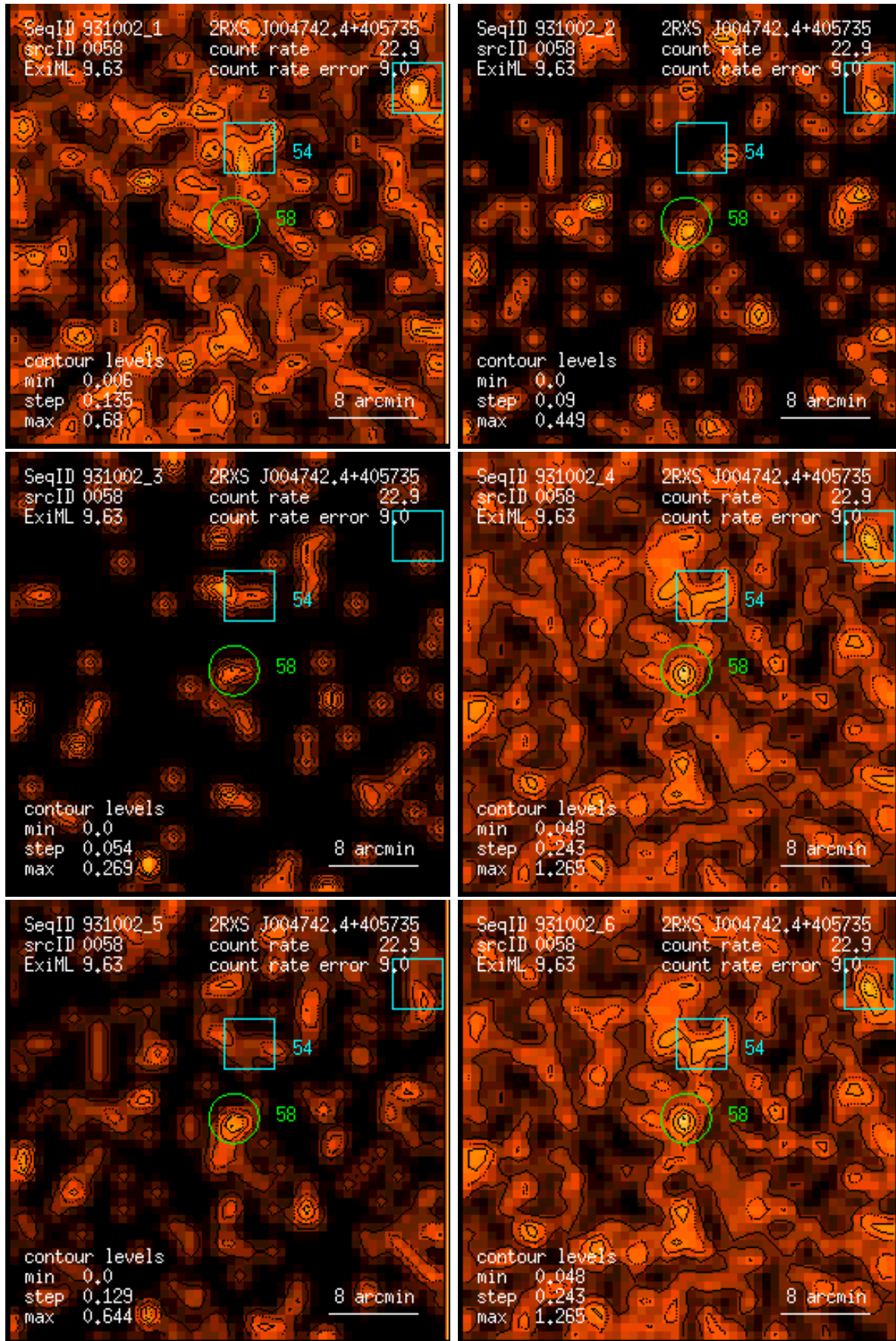
Figure 58: RASS 931002: detection 0058: band rate images, Gaussian filter: (1) PSPC channels 11 – 41, (2) 52 – 90, (3) 91 – 201, (4) 11 – 235, (5) 52 – 201, (6) 11 – 201. Broad band rates in counts/ks. Band rate contour levels in counts/ks/arcmin 2 .
